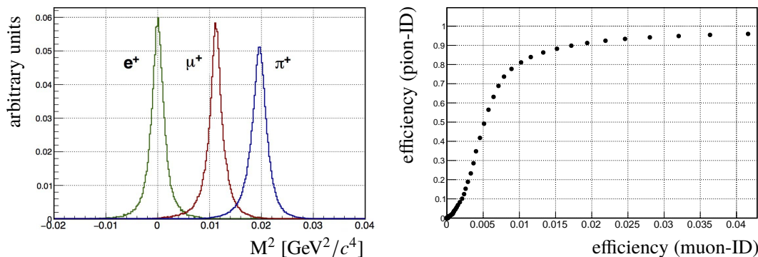
Figure 76. RICH particle identification for track momenta between 15 and 35 GeV/ c . Left: squared particle mass reconstructed using the velocity estimated by the Cherenkov angle measured by the RICH and the momentum measured by the spectrometer, for positrons, muons, and charged pions selected using spectrometer and calorimetric information. Right: pion-ID efficiency versus muon-ID efficiency for different choices of the reconstructed mass range.
