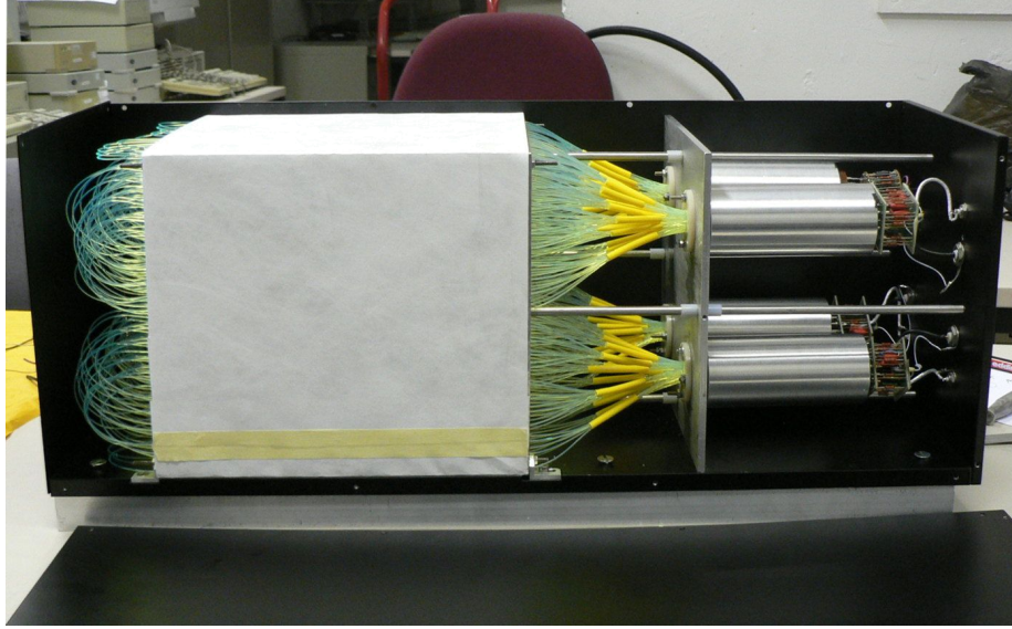
Figure 35. Picture of the SAC after completion of assembly.
