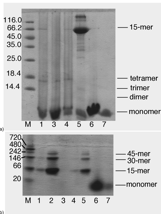
Figure 4. a) SDS-PAGE showing the apparent mass of SDS-resistant species; samples are in the order: M – Marker, 1 – UC-induced at 1.4 mmol dm -3 , 3 – UC-induced sediment at 10 mmol dm -3 , 4 – MAS-induced sediment at 8 mmol dm -3 , 5 – MAS-induced sediment at 2 mmol dm -3 , 6 – supernatant from the preparation of sample 1-2, 7 – monomer. The tetramer band (18 kDa) is evident in samples 1,3,4, while the sample 5 shows the marked presence of heavier species as 68 kDa and approximately 146 kDa. b) Native gel electrophoresis showing the apparent mass of oligomers; samples are in the order: M – Marker, 1 and 2 – UC-induced at 1.4 mmol dm -3 , 3 – UC-induced sediment at 10 mmol dm -3 , 4 – MAS-induced sediment at 8 mmol dm -3 , 5 – MAS-induced sediment at 2 mmol dm -3 , 6 – supernatant from the preparation of sample 1-2, 7 – monomer. The most abundant species in samples 1,2 and 4,5 is the 68 kDa oligomer (15-mer), in agreement with the theoretical predictions, with other two major bands at about 146 and 207, consistent with the 30-mer and 45-mer respectively. In sample 3 no soluble species is observed.
