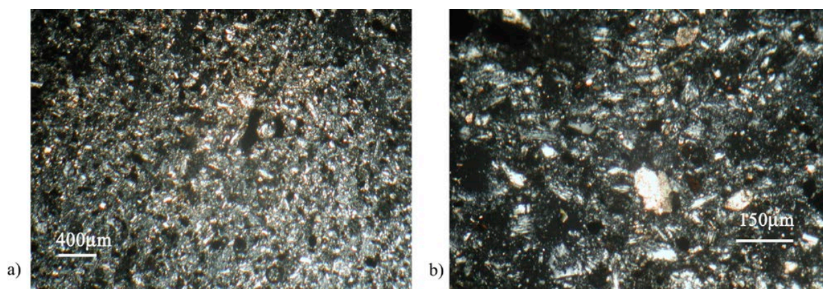
Figure 6. Product L, sample 18 – a) Cross nicols image: general view of the plaster with gypsum in the binder and in the aggregate; b) Cross nicols image: particular of the binder of dark colour, constituted by gypsum; it is visible aggregate, with prevalence of gypsum and trace of quartz and calcite (in colour brown in the top of image).
