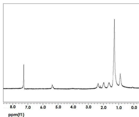
Figure 5. Product E, sample 7 - a) FT-IR spectrum; b) Soluble fraction in \text{CDCl}_3 , ^1\text{H-NMR} ( \text{CDCl}_3 ) spectrum.
