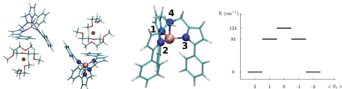
Fig. 1 Left panel: the structure of the [Na(tpa Ph )Fe] - 3 DME (DME = dimethoxyethane) unit cell. Central panel: zoom in on the molecular structure of [(tpa Ph )Fe] - . The color code is: Fe pink, N blue, C green, O red, Na brown and H white. The equatorial N atoms are marked by the labels 1 to 3 and the axial N atom by 4. Right panel: spin energy levels diagram obtained from the diagonalization of the computed spin Hamiltonian.
