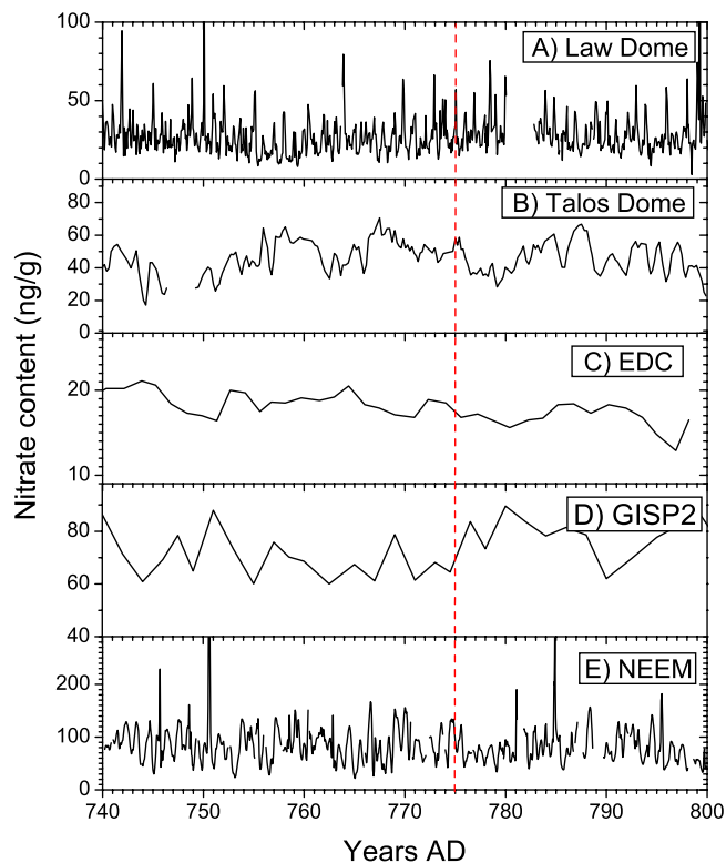
Figure 2. Measured concentrations of nitrate in several polar ice cores around 775 AD (see Table S1). Panel A: Law Dome, data with about monthly resolution; dating uncertainty is \pm 7 year. Panel B: Talos Dome, data with quarterly resolution. Panel C: Annual data from EPICA Dome C. Panel D: data from GISP2. Dating uncertainty of these three data sets can be also on the order of a several years. Panel E: NEEM, data with about 20 samples per year time resolution; note that the \text{NO}_3 data is from the NEEM main core, while the ^{10}\text{Be} peak at 774–775 was derived on a shallow core close-by (NEEM-S1). The relative dating uncertainty of these two neighboring cores should not be more than a few years and clearly smaller than 7 years. Within this uncertainty no \text{NO}_3 peak is found in the NEEM main core. The vertical red dashed line depicts the proposed year of the SEP event.
