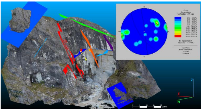
Figure 10. 3D view of the colored point cloud of the Carrara marble quarry with the main extracted discontinuities. The inset shows the stereonet plot of the identified discontinuities.
