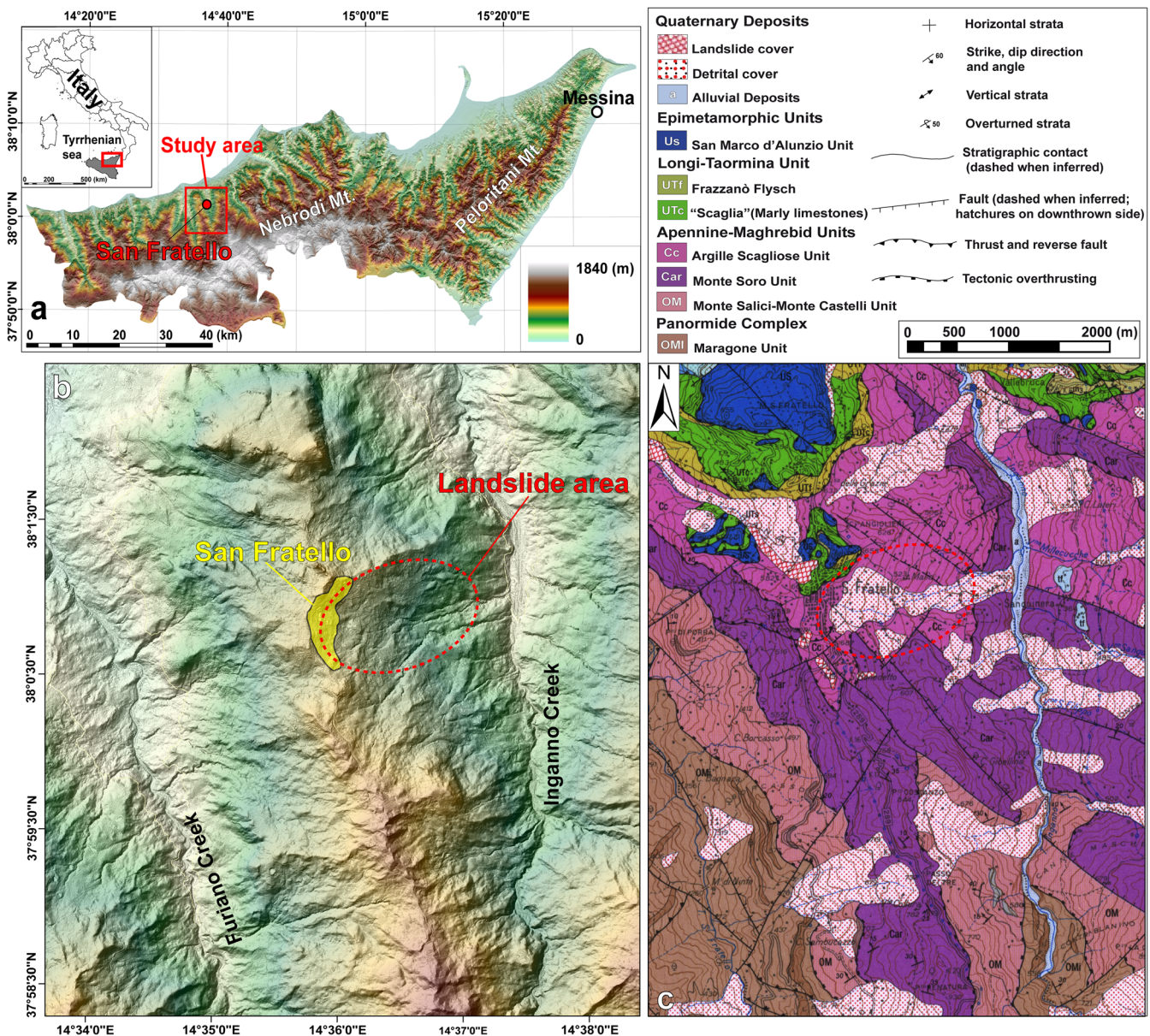
Fig. 1 a Location of the study area with digital elevation model of the Messina Province showing the study area. b DEM of the San Fratello area (2 -m cell resolution). c Geological setting of the study area (dotted red oval enhances the town sector; modified after Lentini et al. 2000)
