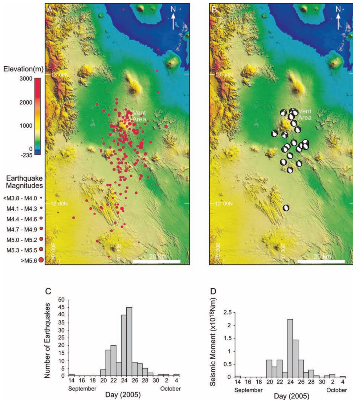
Figure 8. 90 m SRTM Digital elevation model of the Dabbahu Magmatic Segment and surrounds showing (A) the distribution of earthquakes reported by NEIC between 2005 September 14 and October 4 (red circles scaled according to magnitude), and (B) earthquake focal mechanisms determined by Harvard CMT. The histograms show (C) earthquake frequency per day and (D) combined seismic moment released per day.
