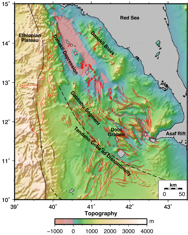
Fig. 2. Structural map of the Afar Depression, showing fault traces from Central Afar (Manighetti et al., 2001) and Northern Afar. Major surface, Pliocene–Recent faults are in red. Fault traces are available in the supplementary material. (For interpretation of the references to colour in this figure legend, the reader is referred to the web version of this article.)
