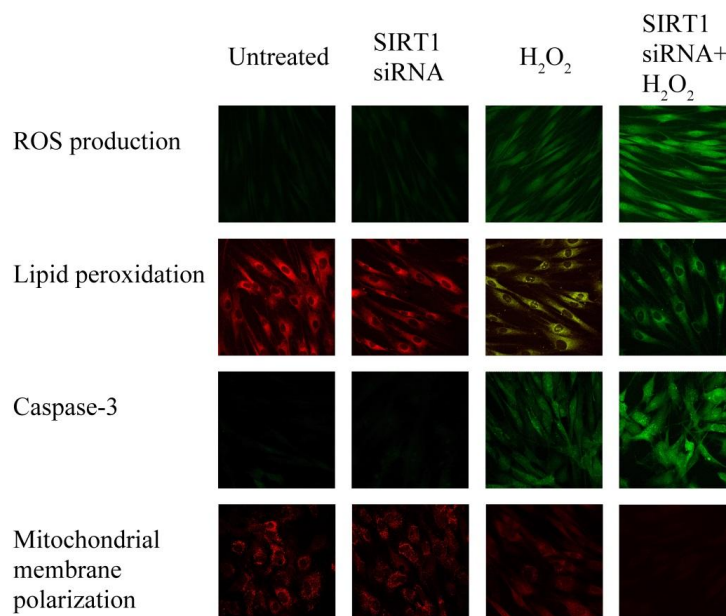
Figure 6. SIRT1 effects in oxidative stress protection. ROS production, lipid peroxidation, caspase-3 activity and mitochondrial membrane polarization were measured by confocal microscopy (63× magnification) in untreated and in SIRT1 siRNA-treated control fibroblasts, challenged or not with H 2 O 2 (500 µM for 3 h) to elucidate the role of SIRT1 in oxidative-mediated cell injury. Fibroblasts were obtained from healthy skin ( n = 4 biopsies). These parameters were measured in untreated and in SIRT1 siRNA-treated control fibroblasts, challenged or not with H 2 O 2 (500 µM for 3 h).
