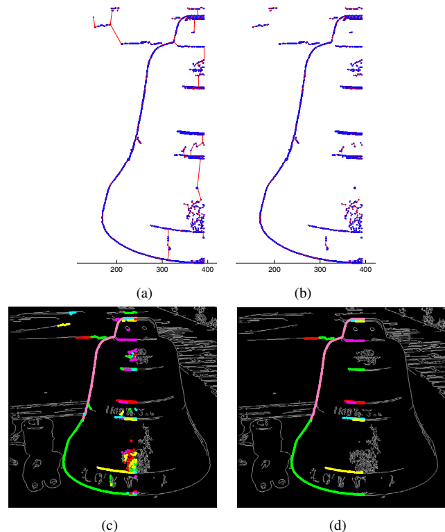
Fig. 3. (a): the EMST of the original image (finer pyramid level). (b): arc removal from branching points. (c): the curves resulting from arc removal. (d): the curves resulting after saliency thresholding.
