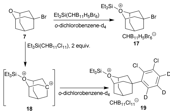
Scheme 6 Reactions of 5-bromo-2-oxaadmantane with trialkylsilylium carborane reagents.
