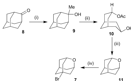
Scheme 2 Synthesis of 5-bromo-2-oxaadmantane 7 . (i) MeMgBr, Et 2 O, 96%; (ii) TFAA, H 2 O 2 , –25 °C, 86%; (iii) 98% H 2 SO 4 , 98%; (iv) 50% NaOH, CBr 4 , BTEAC, CH 2 Cl 2 , 40 °C, 39%.
