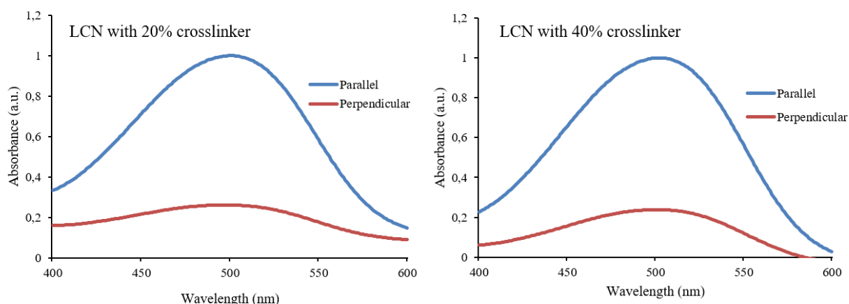
Figure S4. Polarized absorption spectra of LCNs with planar homogeneous alignment recorded respectively in parallel and perpendicular directions with respect to the nematic director.
