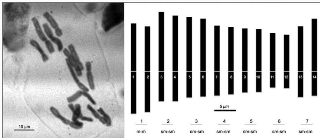
Figure 6. Chromosome metaphase plate and idiogram of G. scipetarum subsp. eddae showing 2n = 2x = 14 and chromosome morphology.
