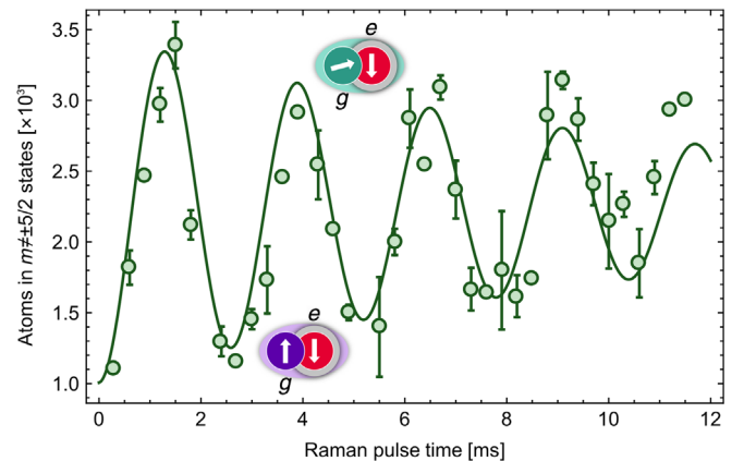
FIG. 6. Rabi oscillation on the bound-to-bound Raman transition peak performed at B = 150 G and a 3D lattice depth s_f = 30 . The Raman light coherently flips the ground-state nuclear-spin component of the molecules between the m = +5/2 state and m = +1/2 state, with a decay time constant of 12(3) ms.
