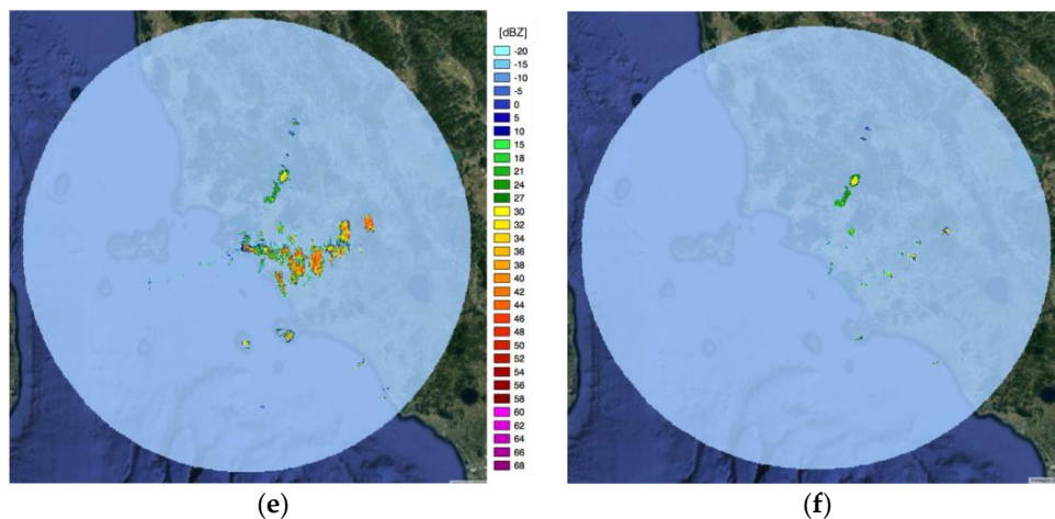
Figure 5. PPI radar scans at an elevation of 1.5^\circ for 23 May 2016, 09:00 UTC, without ( left panels ) and with ( right panels ) the application of the sea and ground clutter removal algorithms for the radars of Livorno ( a,b ); Elba ( c,d ); and Castiglione della Pescaia ( e,f ).
