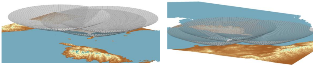
Figure 2. Different overviews of the 3D geolocation of the Plan Position Indicator (PPI) conical scans geometry for the three X-band radars. Elevation is 5^\circ .
