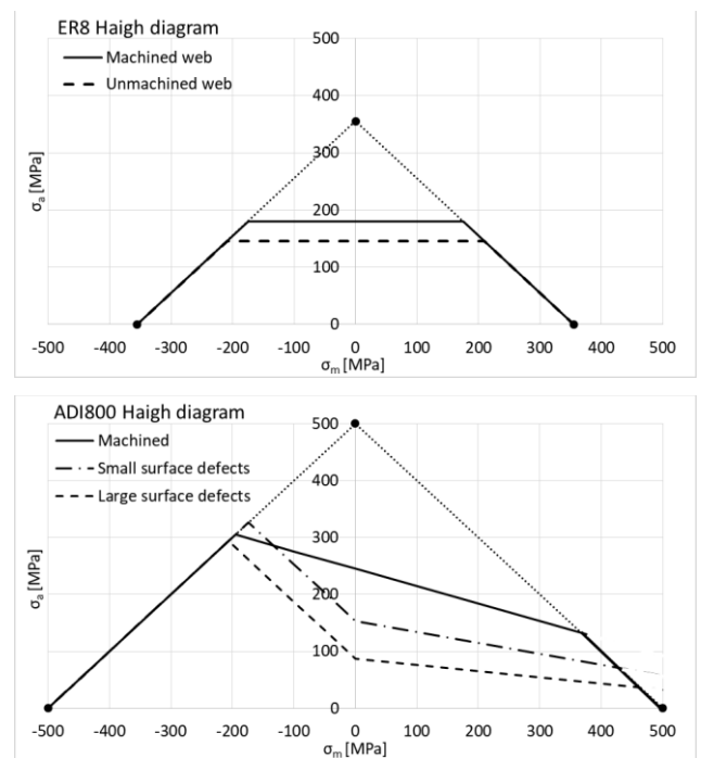
Fig. 7 Haigh diagrams for ER8 steel grade used for monobloc wheels (top) and for ADI800-10 used for the casted wheel centre (bottom).
