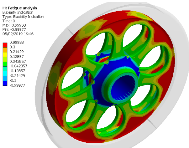
Fig. 6 Bixiality index for the ADI wheel centre with fitting loads and external loads (case 2). Values near zero corresponds to uniaxial stresses.
