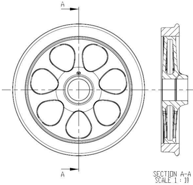
Fig. 1 New tired wheel with ADI casted wheel centre and steel tyre designed as replacement the ALn668 DMU original wheel.
