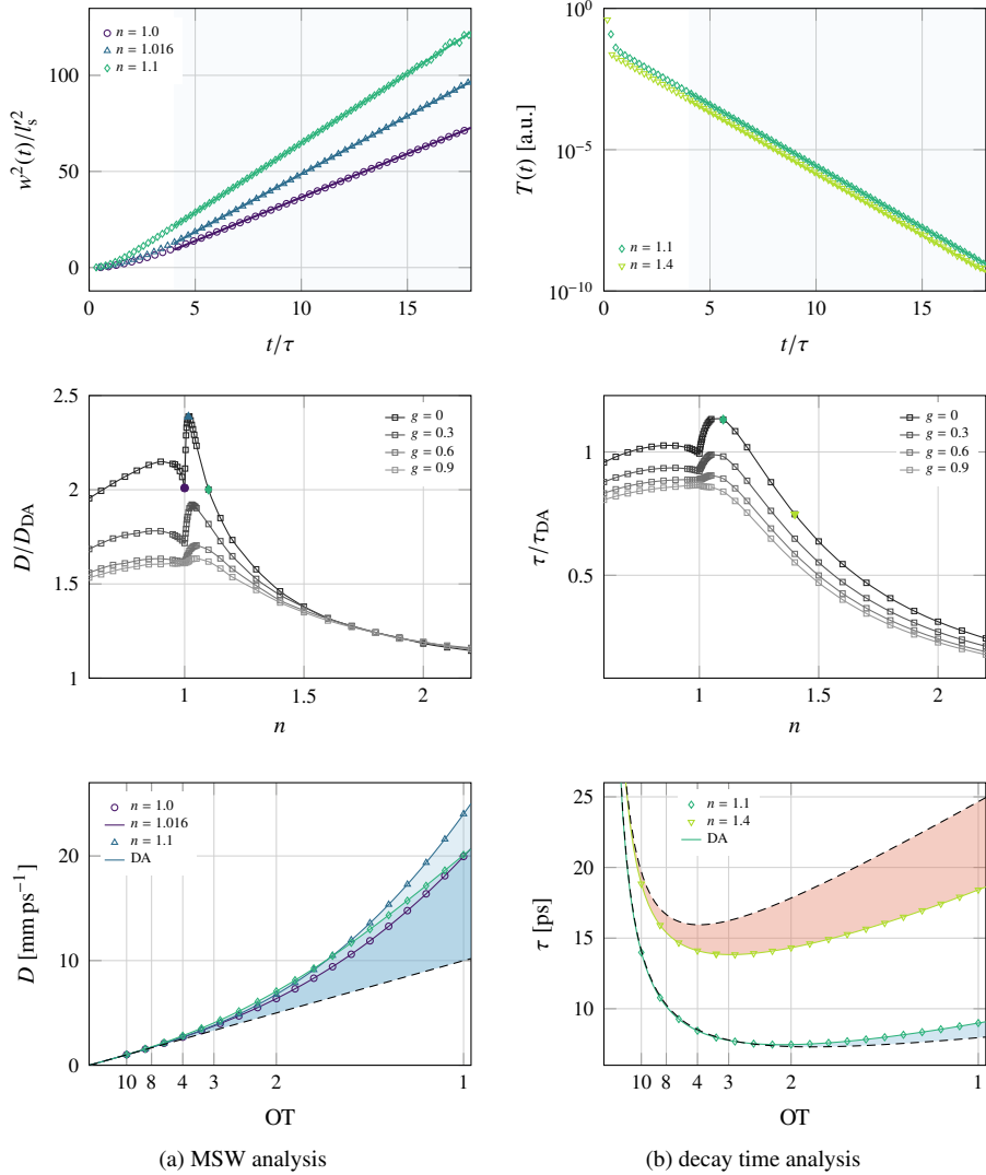
Figure 6.1. From top to bottom: MSW expansion rate and decay time for a slab configuration with l_s^* = L_0 , g = 0 and different refractive index contrasts, exhibiting (a) a perfectly linear growth and (b) a monoexponential decay after a short transient. Dependence on n and g of the diffusion coefficient D and decay constant \tau as inferred from a linear fit of w^2(t \geq 4\tau) and \log T(t \geq 4\tau) for different samples with OT = 1 . Solid points represent the values retrieved from the fits shown in the upper panel. Absolute positive (blue) and negative (red) deviations with respect to the DA prediction are shown in the lower panels for different optical thicknesses. Solid lines serve as guides to the eye.
