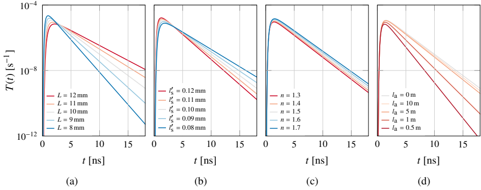
Figure 2.9. Dependence of the integrated transmittance T(t) in the diffusive approximation on (a) the thickness of the slab L , (b) the reduced scattering mean free path l'_s , (c) the refractive index contrast n and (d) the absorption length l_a . Each parameter contributes differently to change both the amplitude and the shape of the profile.
