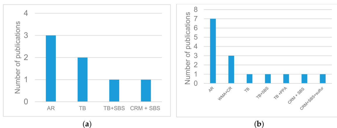
Figure 11. Comparison of rheological properties: (a) the number of studies reporting a higher value of the complex modulus for each CRM binder compared to traditional binder; and (b) the number of studies reporting a lower value of the phase angle for each CRM binder compared to the traditional binder.
