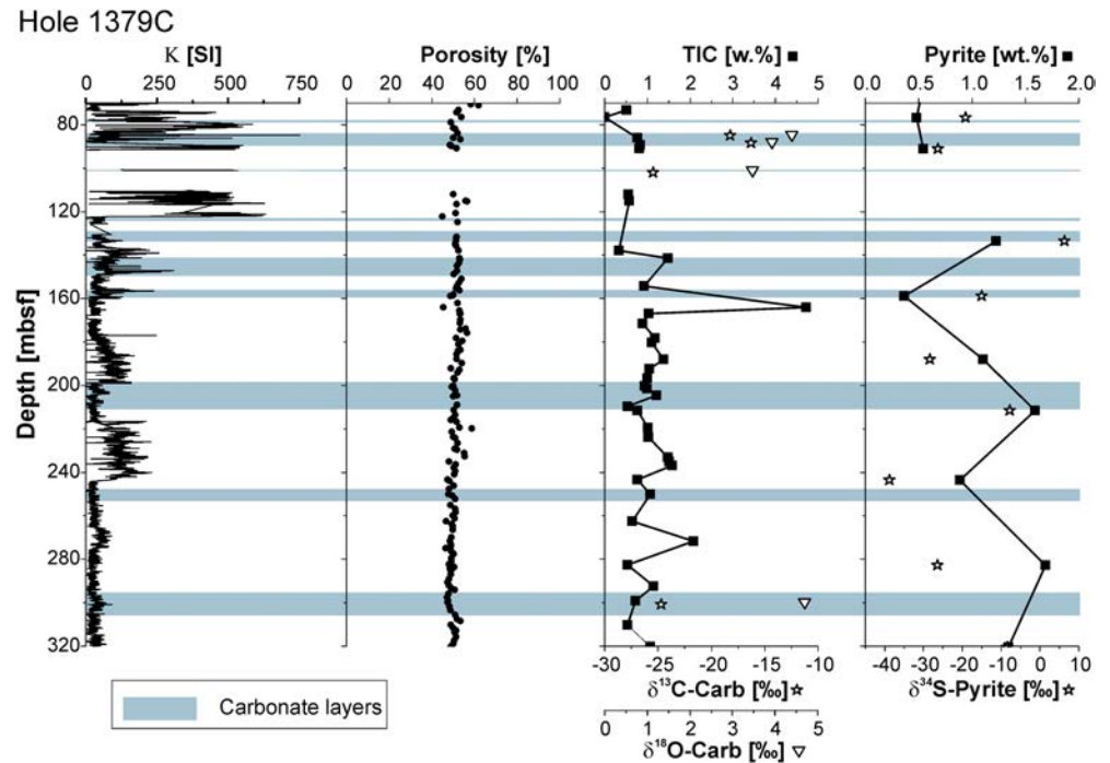
Figure 5. Site U1379 content profiles between 70 and 320 mbsf for the magnetic susceptibility (K), porosity, total inorganic carbon (TIC), pyrite, and its sulfur isotopes ( \delta^{34}\text{S} -Pyrite). The light-blue bars indicate observed carbonate layers (see Vannucchi et al., 2012). It should be noted that most samples for TIC analyses were taken outside observed carbonate layers based on sedimentary description (see also Site U1379 description in Vannucchi et al., 2012).
