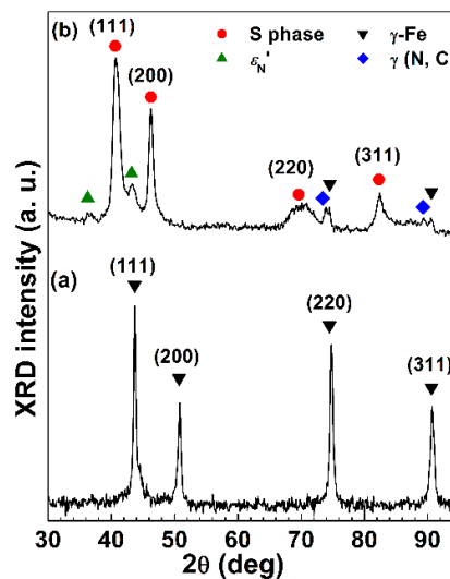
Figure 5. X-ray diffraction patterns of AISI 316L samples: (a) untreated; (b) plasma nitrided at 380^\circ\text{C} , 340 Pa, 3 h (Bragg-Brentano configuration, Cu K\alpha radiation). For further experimental details, see [70].
