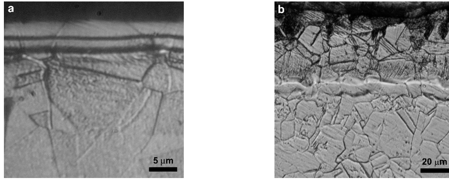
Figure 4. Cross-section (a) and tapered section ( \sim 10^\circ ) (b) of an AISI 316L sample plasma nitrided at 380^\circ\text{C} , 340 Pa, 3 h. For further experimental details, see [70]. (Etchant: acetic glyceric acid (3 mL HCl, 2 mL \text{HNO}_3 , 2 mL acetic acid, 1 drop of glycerol; in (b) the marker refers to the length in the tapered section)).
