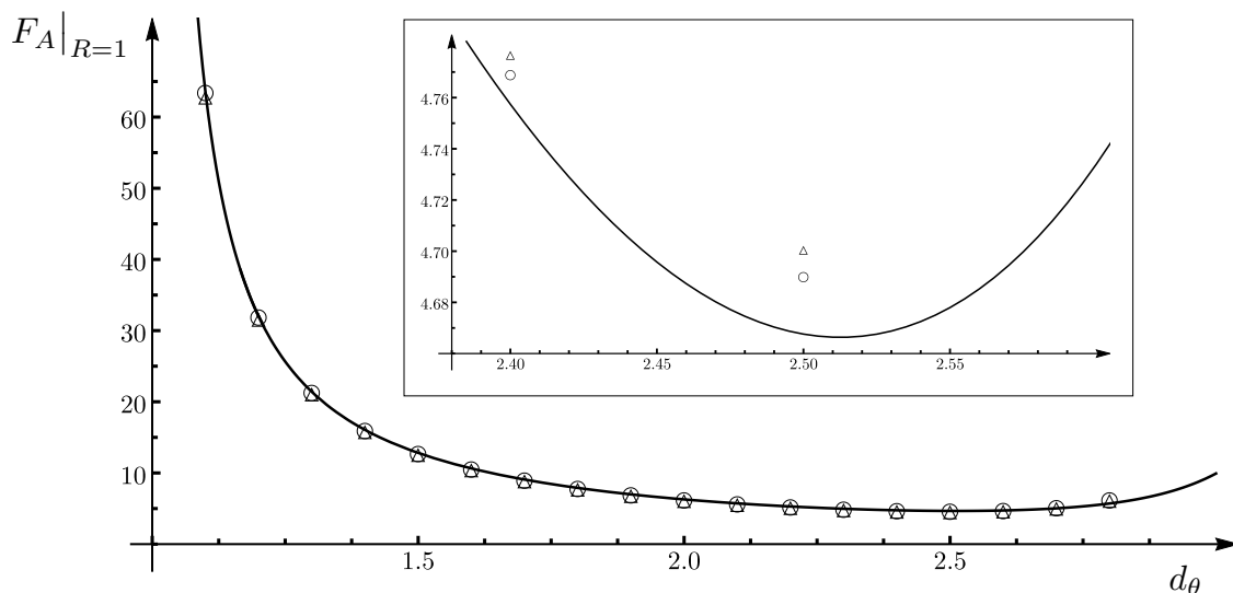
Figure 2. Finite term F_A in terms of 1 < d_\theta < 3 for minimal surfaces anchored to a disk of radius R = 1 in the hvLif_4 geometry (2.21) at t = \text{const} . The solid line is found by first solving numerically (with Wolfram Mathematica) the differential equation (5.15) and then plugging the resulting radial profile into (5.17). The data points labelled by the empty circles and the empty triangles have been obtained with Surface Evolver through the two formulas in (5.20) respectively. The inset contains a zoom close to the minimum of the curve, that corresponds to (d_\theta, F_A) \simeq (2.52, 4.67) .
