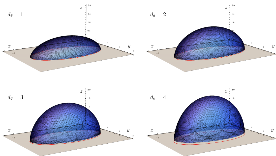
Figure 1. Minimal area surface obtained with Surface Evolver whose area provides the holographic entanglement entropy of an ellipse A delimited by the red curve. The minimal surface is embedded in a constant time slice of the four dimensional hyperscaling violating Lifshitz spacetime (2.1), whose metric depends on the hyperscaling parameter d_\theta .
