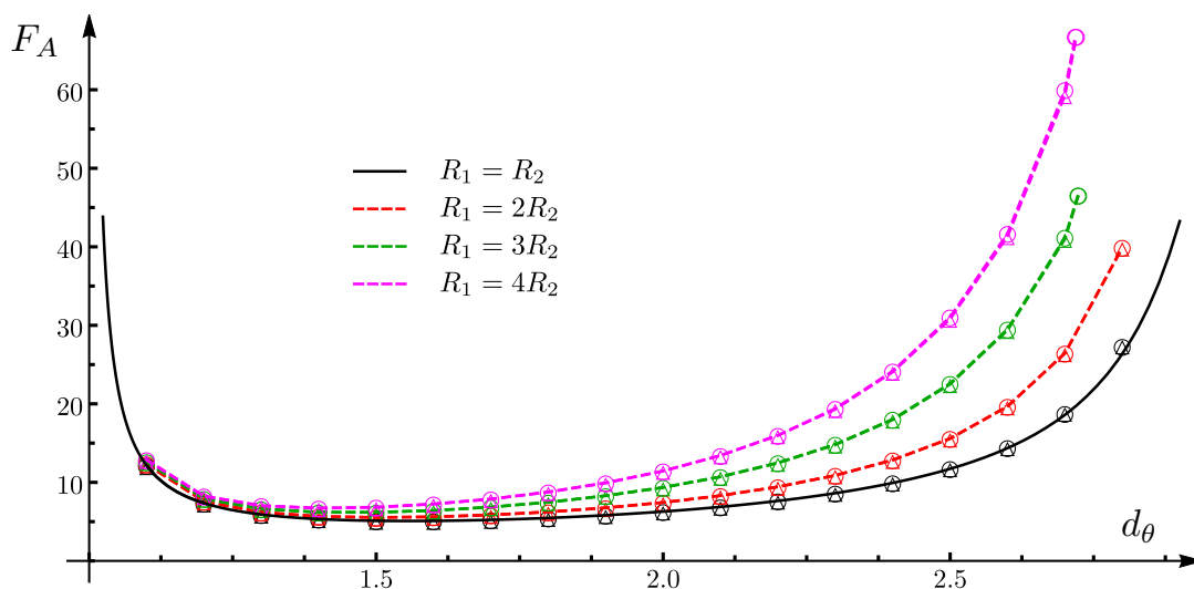
Figure 6. Finite term F_A in terms of d_\theta in the range 1 < d_\theta < 3 for minimal surfaces in hvLif_4 anchored to ellipses A having fixed perimeter P_A = 1 . Different colours correspond to ellipses with different eccentricity. The data points have been obtained with Surface Evolver in the two ways described in (5.20) (the markers have been assigned as in the previous figures). The solid black curve, that corresponds to the disk, is the curve reported in figure 2 multiplied by (P_A/(2\pi R))^{2-d_\theta} .
