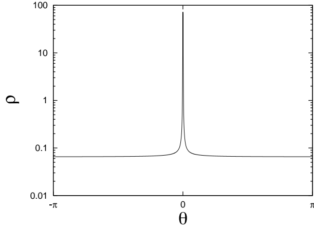
Figure 6: A typical mass density distribution \rho(\theta) for \varepsilon = 10^{-5} and U = -20.0 , in the negative specific heat region.
