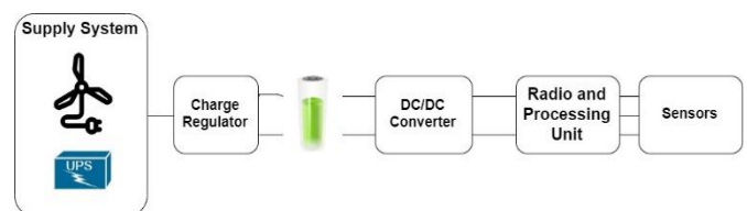
Figure 4. Block diagram of the sensor node.
