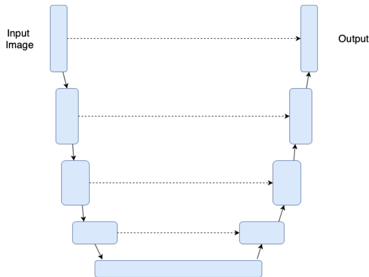
Figure 5. General schema of Unet architecture: input and output have the same size.
