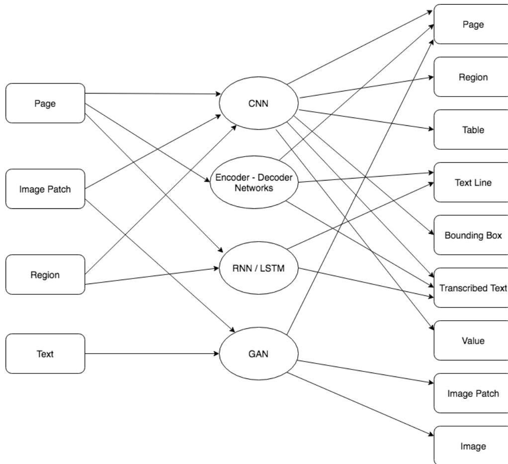
Figure 7. Most frequent Input-Output combinations and related Neural Networks architectures.
