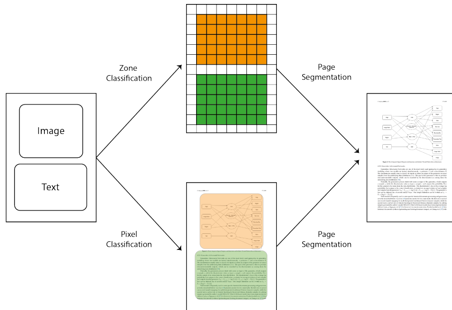
Figure 1. Zone (or patch) classification compared to pixel classification.
