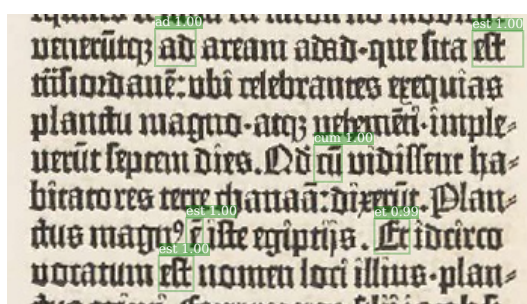
Figure 3. Keyword spotting in a fragment of Gutenberg's Bible [21].
