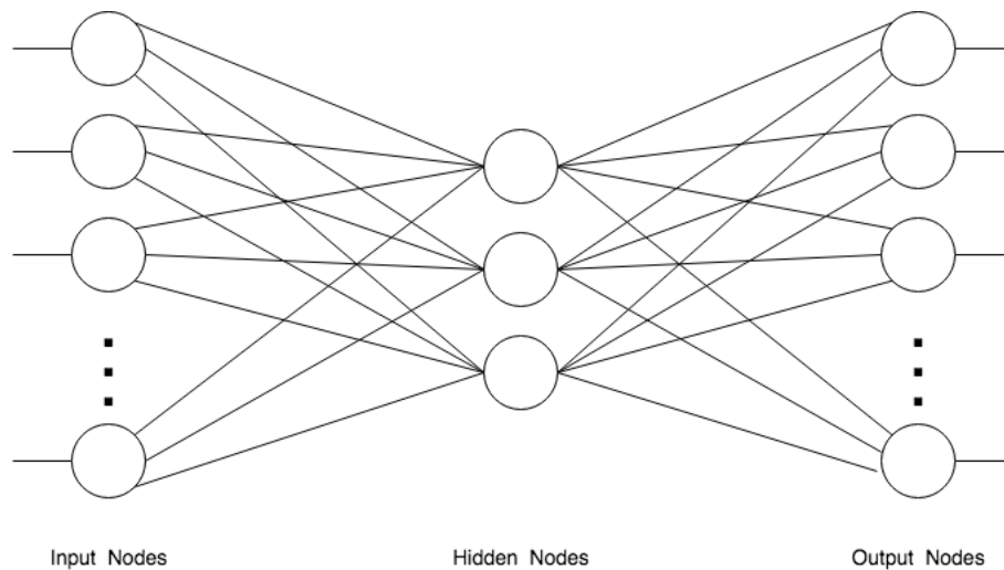
Figure 6. Autoencoder architecture: input and output have the same size.
