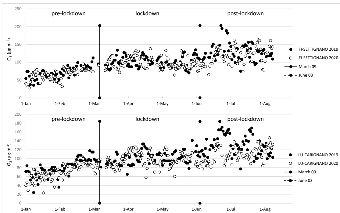
Figure 5. The daily mean concentration of O 3 (μg·m -3 ). The area between the vertical bars in each graph indicates the duration of the lockdown duration.
