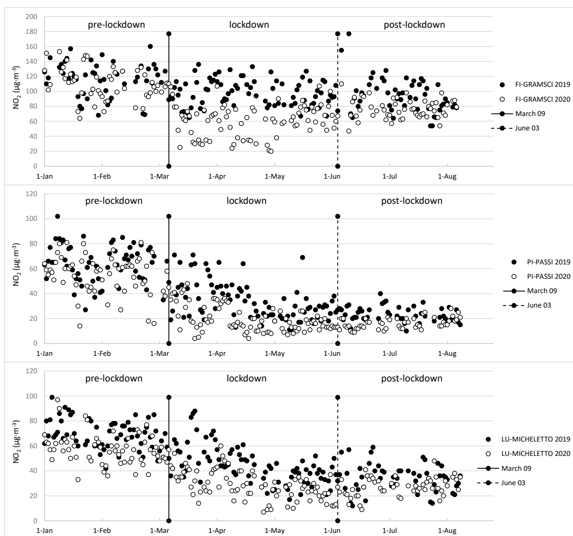
Figure 4. The daily mean concentration of NO 2 (μg·m -3 ). The area between the vertical bars in each graph indicates the duration of the lockdown.
