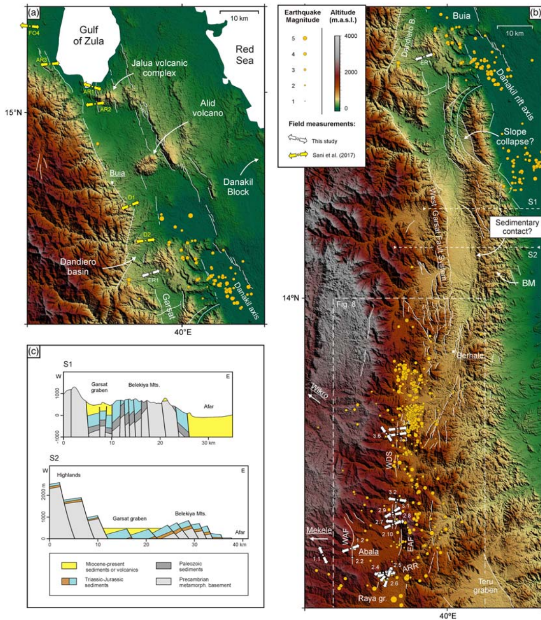
Figure 5. Detailed maps of (a) the Buia graben and (b) Garsat graben. AAR: Abala-Raya Ridge, EAF: East Abala Fault, BM: Bekekiya Mountains, WAF: West Abala Fault, WB: Wikro Basin WDS: Wikro Dike Swarm. Note the crescent-shaped depression at NE edge of the Garsat graben, which Chorowicz et al. (1999) interpret as a slope collapse structure. Earthquakes are shown by yellow circles, scaled for magnitude, interpreted faults by white lines. Background topography is derived from ASTER data (90 m resolution). For locations, see Figure 3b. (c) Two contrasting structural interpretations for the SE Garsat graben margin, S1 being the interpretation by Kazmin et al. (1978) involving a faulted contact, whereas Williams (2016) proposes a halfgraben architecture with a sedimentary contact on the basis of data from Garland, (1980) (S2). Hagos et al. (2016) and Le Gall et al. (2018) support the latter option. (Approximate) section locations are indicated in (b).
