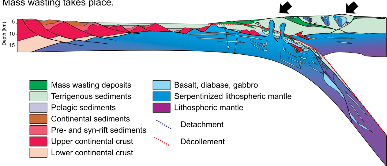
Figure 2. Model of structure and evolution of the exhumation and diapirism of serpentinized peridotites from rifting to subduction. (A) Evolved structure at magma-poor hyperextended margin, adapted from the Galicia margin example (offshore western Spain; modified from Boillot et al. 1995) and slow-spreading rifted margin environment reconstructed from the western Alps and Corsica for the western Tethys (modified from Lagabrielle et al., 2015). (B) Subduction complex with active emplacement of serpentinite diapirs in the inner forearc, embedded shorn diapiric masses in the external part of the prism, and possible mass wasting (marked as dark green units) that reworks some blocks, either as they are emplaced or post-emplacment.
