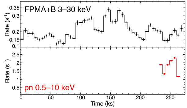
Figure 1. Top: Combined FPMA and FPMB background subtracted light curve in the 3–30 keV energy band showing the rapid variability during the 270 ks observation. Bottom: EPIC-pn light curve of Ton S180 during the last 30 ks of the observation. For clarity the time bin of the light curves from both observatories correspond to the length of one NuSTAR orbit, i.e., 5814 s.
