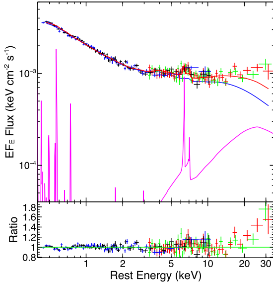
Figure 9. Same as in Fig. 8 (right panel), but with the addition of a distant reflector component modelled with xillver (magenta) to the blurred reflection (blue), here reproduced by relxillCp , in order to reduce the residuals at E > 10 keV. Despite the considerable statistical improvement, the best-fit model still struggles to properly account for the Fe K and hard X-ray band (see Table 4 for the model parameters).
