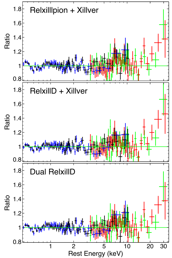
Figure 10. Data/model ratio plots corresponding to three different fits carried out on the 2016 XMM-Newton and NuSTAR data of Ton S180 with different flavours of the relxill relativistic reflection models. Relativistic reflection alone, regardless of which version of relxill we use, cannot self-consistently account for the 0.4–30 keV spectra leading to significant residuals in the iron K band and above 10 keV.
