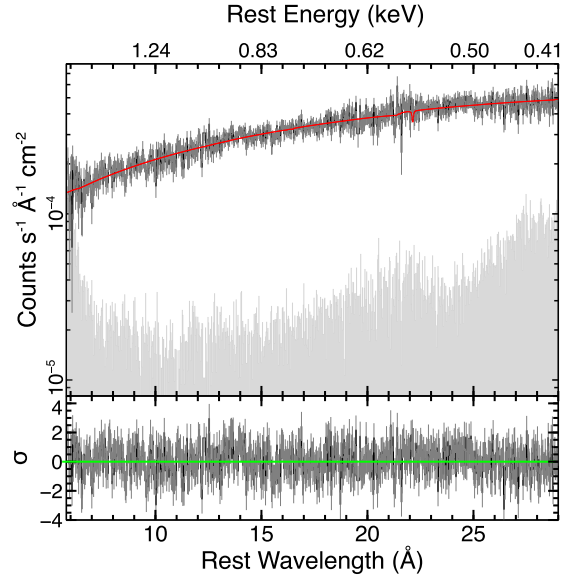
Figure 4. Top: Stacked background subtracted RGS 1+2 spectrum from the 2000, 2002, 2015 and 2016 XMM-Newton observations of Ton S180. The best-fit (power-law modified by Galactic absorption) model is overlaid in red and the background level is shown in grey. Bottom: corresponding residuals of the data points compared to the best-fit model, in \sigma units. The soft X-ray spectrum is largely consistent with a simple power law with a steep photon index of \Gamma = 2.93 \pm 0.02 .
