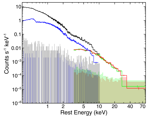
Figure 2. Background subtracted EPIC-pn (black), MOS 1+2 (blue), FPMA (red) and FPMB (green) spectra between 0.3–79 keV and the corresponding background levels of the joint 2016 XMM-Newton and NuSTAR observation of Ton S180. It is clear the the background contribution dominates above \sim 30 keV. We will use the 0.4–30 keV energy band for the X-ray analysis in this paper.
