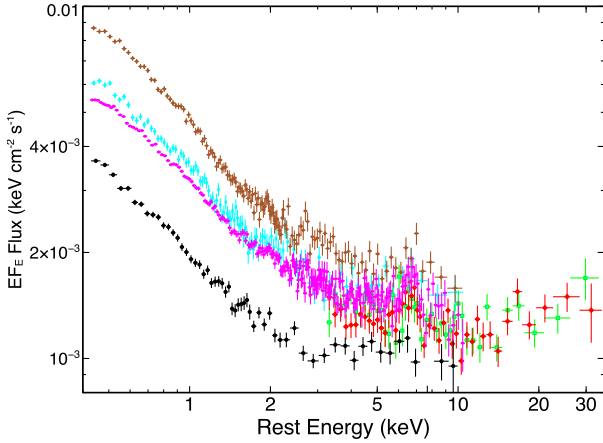
Figure 3. Background subtracted Ton S180 spectra corresponding to the 2016 XMM-Newton and NuSTAR EPIC-pn (black), FPMA (red) and FPMB (green). Note that the average intensity of the source over the entire NuSTAR observation was about 30 per cent larger than during the simultaneous coverage with XMM-Newton (see Fig. 1). Also the EPIC-pn spectra from 2000 (brown), 2002 (cyan) and 2015 (magenta) are shown for comparison.
