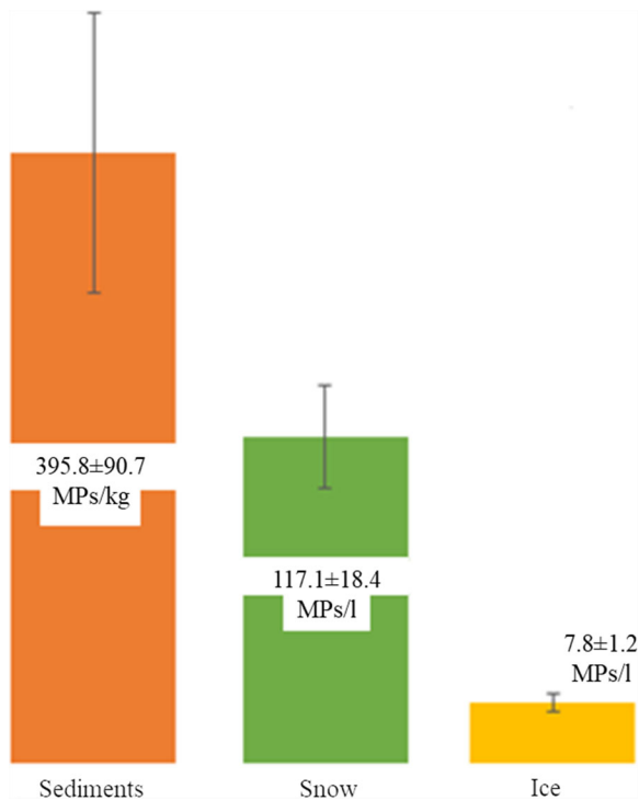
Fig. 10 MP average concentrations found in sediment, snow, and ice
