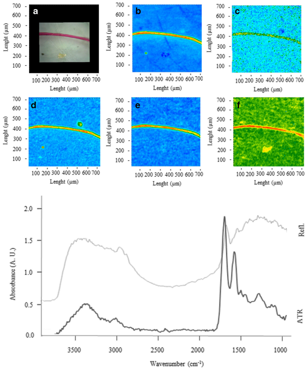
Fig. 9 FTIR spectra, visible, and IR imaging of a wool fibre. (Top left) Visible light map of the filter substrate, with a plastic fibre lying on it (a). (Top right, centre, and bottom panels) 2D FTIR imaging maps, where the intensity of the following bands was mapped: 3460 (OH stretching) (b), 3047 (amide B stretching) (c), 2912 (CH stretching) (d), 1697 (e) (amide I stretching), and 1558 \text{cm}^{-1} (amide II stretching) (f). The chromatic scale of each map
