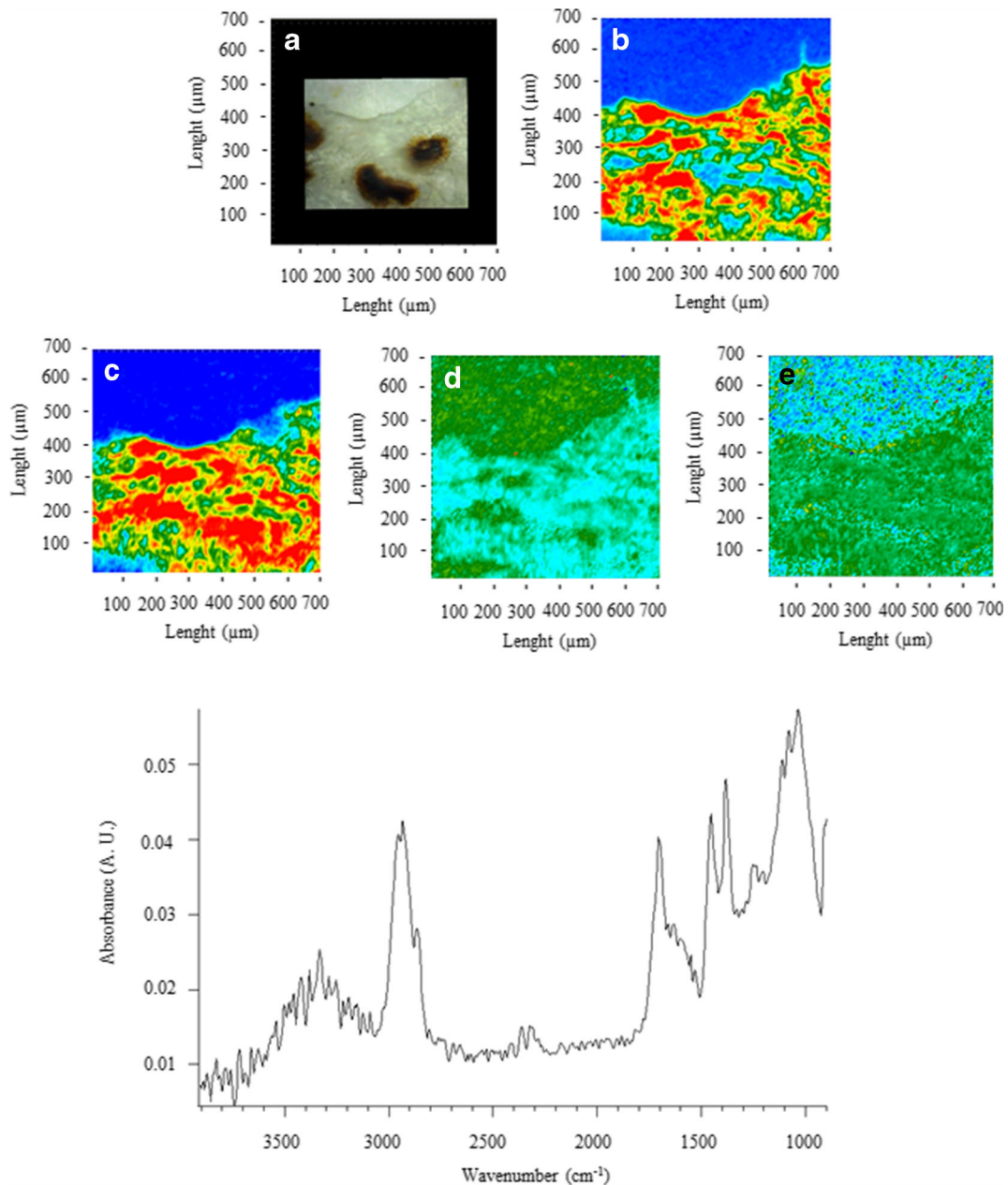
Fig. 4 FTIR spectra, visible, and IR imaging of a polypropylene fragment. (Top left) Visible light map of the filter substrate, with a plastic fragment lying on it (a). (Top right and centre panels) 2D FTIR imaging maps, where the intensity of the following bands was mapped: 2931 (CH stretching) (b), 1715 (C=O stretching) (c), 1458 ( \delta_{as} CH 2 ), and 1377 ( \delta_s CH 3 ) cm -1 . The chromatic scale of
