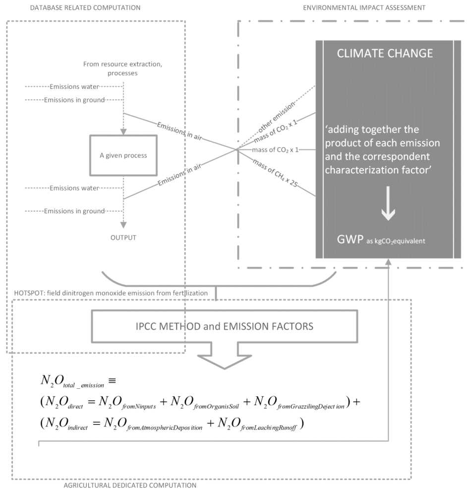
Figure 3. Overview of the methodological framework adopted in the study (GWP = global warming potential, indicator of the impact category “Climate Change”).
