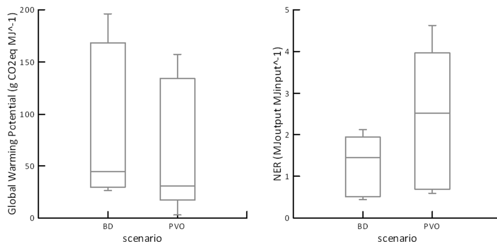
Figure 5. Uncertainty assessment of the two considered camelina scenarios (BD, biodiesel; PVO, pure vegetable oil) for global warming potential and net energy ratio (NER), by means of quartiles distribution around the median values (conventional boxplot) computed by varying grain yield and seed oil content according to the estimated variability of field performances.
