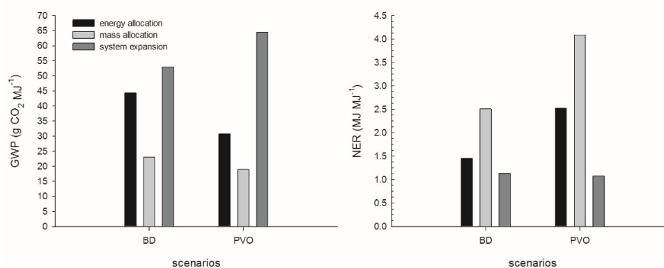
Figure 6. Sensitivity assessment of the two considered camelina scenarios (BD, biodiesel; PVO, pure vegetable oil) as the allocation procedures vary.
