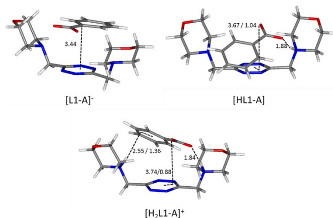
Figure 8. Calculated solution conformations of L1 complexes with benzoate (A - ) in solution. Distances in Å. Parameters for anion-π contacts given as plane/offset values.
