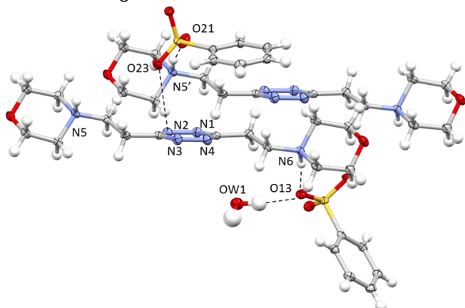
Figure 4. ORTEP drawing and details of the crystal packing of the \text{H}_2\text{L}_2(\text{C}_6\text{H}_5\text{SO}_3)_2 \cdot \text{H}_2\text{O} crystal structure. Selected contacts are shown.
