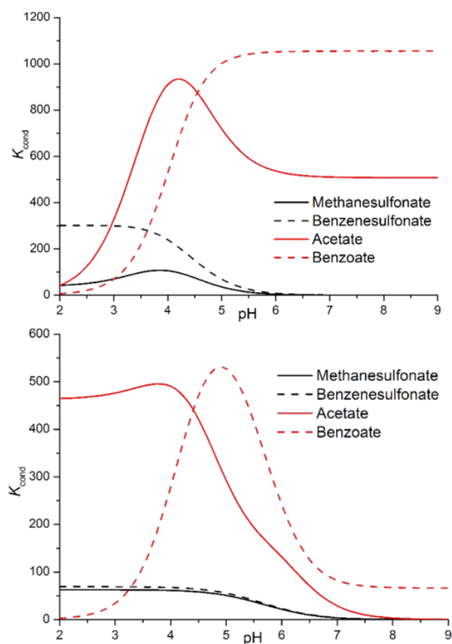
Figure 5. Conditional stability constants for complexes of L1 (top) and L2 (bottom) with the series of monovalent anions
