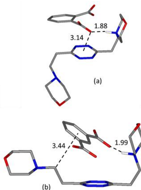
Figure 10. Calculated most stable conformations in solution of HL 2 + complexes with phthalate (a) and (b) isophthalate dianions, respectively.
