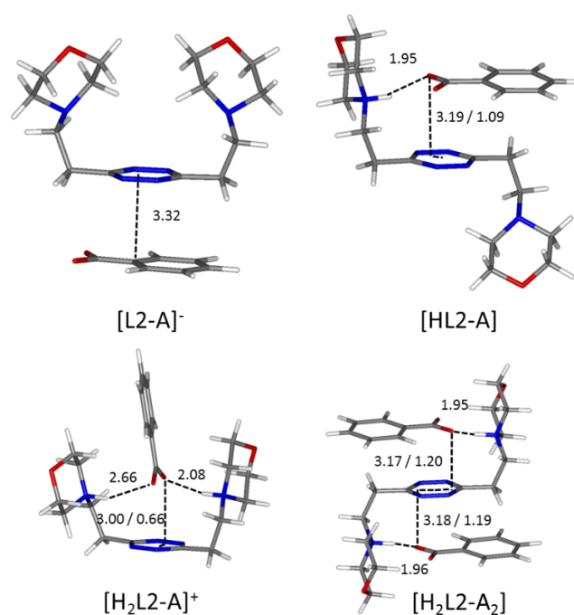
Figure 6. Calculated solution conformations of L2 complexes with benzoate ( \text{A}^- ) in solution. Distances in Å. Parameters for anion- \pi contacts given as plane/offset values.
