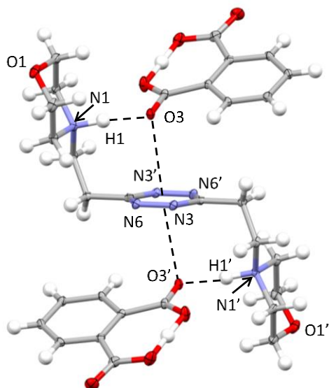
Figure 2. ORTEP drawing of the (H 2 L)(HPhthalate) 2 complex in the (H 2 L)(HPhthalate) 2 ·2H 2 O crystal structure. Selected contacts are shown.
