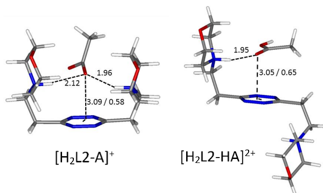
Figure 9. Calculated solution conformations of selected L2-acetate (A - ) complexes in solution. Distances in Å. Parameters for anion- \pi contacts given as plane/offset values.
