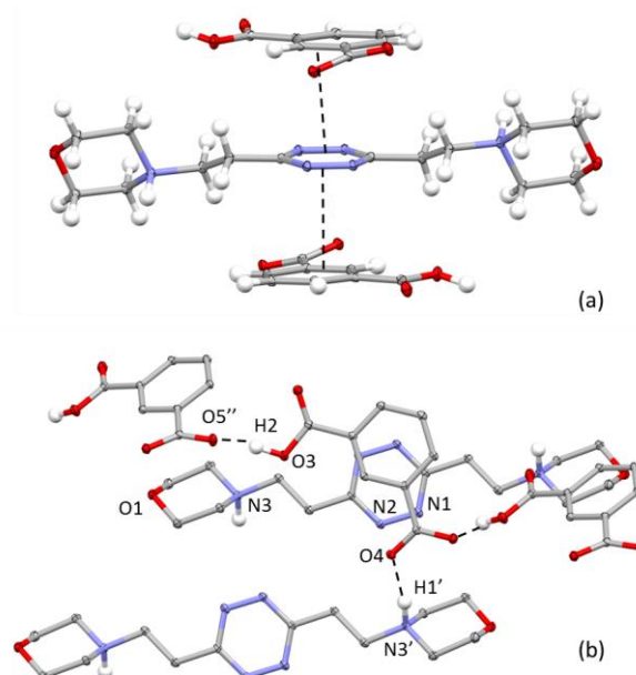
Figure 3. ORTEP drawing of the (H 2 L)(Hisophthalate) 2 crystal structure. (a) lateral view of the complex; (b) details of the crystal packing. Selected contacts shown.
