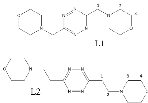
Figure 1. The tetrazine-based ligands L1 and L2.
