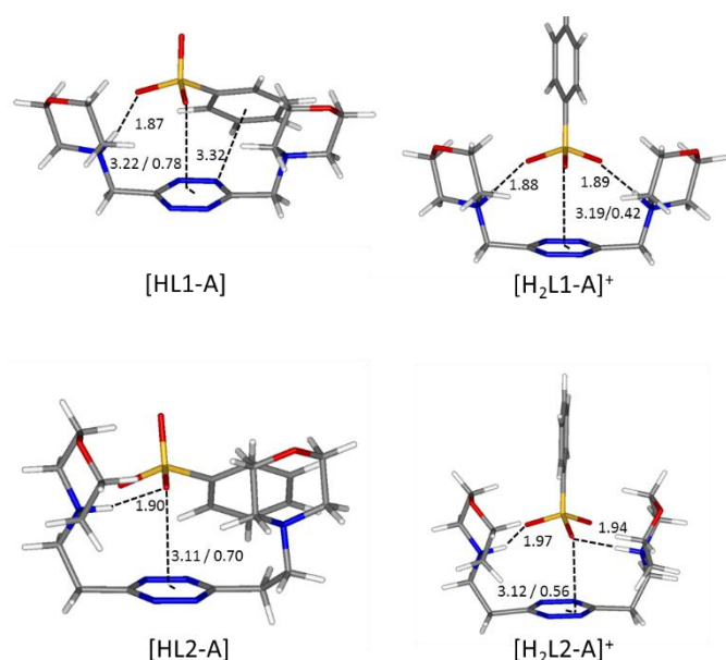
Figure 7. Calculated solution conformations of L1 (top) and L2 (bottom) complexes with benzenesulfonate (A - ) in solution. Distances in Å. Parameters for anion-π contacts given as plane/offset values.
