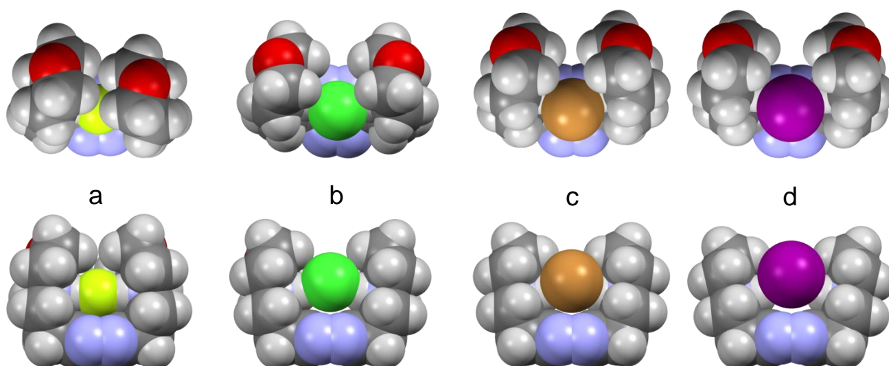
Figure 7. Top (above) and lateral (below) views of the DFT optimized geometries for fluoride (a), chloride (b), bromide (c) and iodide (d) complexes of \text{H}_2\text{L}_2^{2+} in PCM water.
