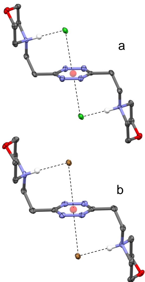
Figure 3. Crystal structures of H_2L_2Cl_2 (a) and H_2L_2Br_2 (b).
