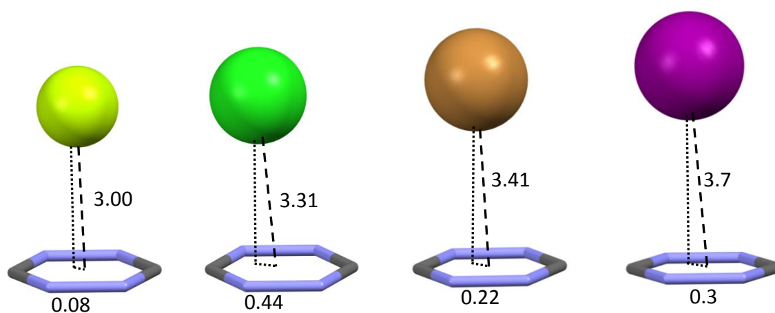
Figure 4. Distances ( \text{\AA} ) of anions from the tetrazine ring centroid and offsets in the crystal structures of H_2L_2F_2 \cdot 3H_2O \cdot CH_3OH , H_2L_2Cl_2 , H_2L_2Br_2 and H_2L_2I_2 \cdot 2H_2O . Data for H_2L_2I_2 \cdot 2H_2O are from ref. 11a.
