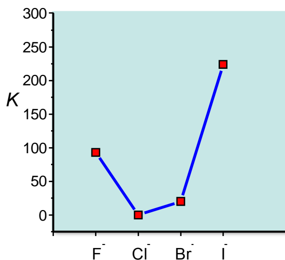
Figure 6. Equilibrium constants ( K ) for the reactions \text{H}_2\text{L}2^{2+} + \text{X}^- = [(\text{H}_2\text{L}2)\text{X}]^+ ( \text{X} = \text{halide} ). For \text{Cl}^- , K was arbitrarily set equal to zero, as it is expected to be close to this value.
