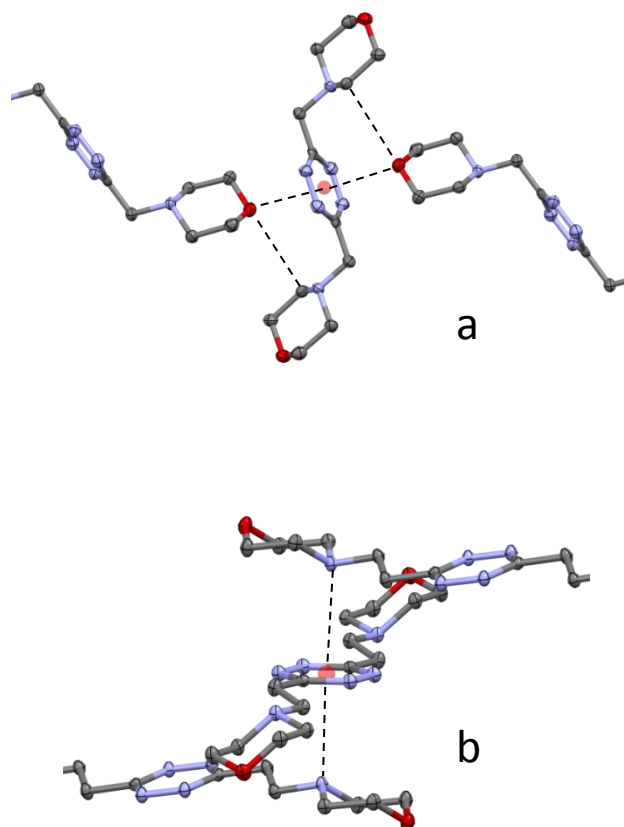
Figure 5. Crystal structures of the free ligands L1 (a) and L2 (b) with details of the packing interaction.
