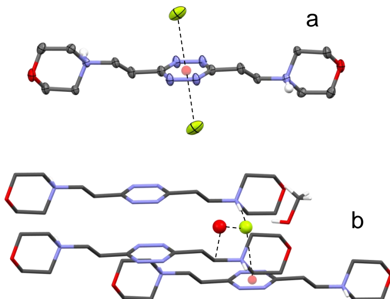
Figure 2. Crystal structure of \text{H}_2\text{L2F}_2 \cdot 3\text{H}_2\text{O} \cdot \text{CH}_3\text{OH} . Details of the \text{H}_2\text{L2F}_2 complex (a) and of the crystal packing (b).
