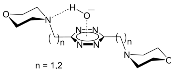
Figure 8. Schematic representation of the hydrogen bond and anion- \pi interactions suggested for [L1(OH)]^- ( n = 1 ) and [L2(OH)]^- ( n = 2 ) complexes.
