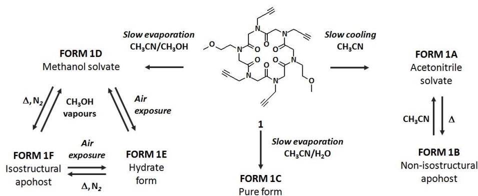
Scheme 1. Crystal forms of cyclo-(Nme-Npa) 2 1 , Nme = N-(methoxyethyl)glycine, Npa = N-(propargyl)glycine.
