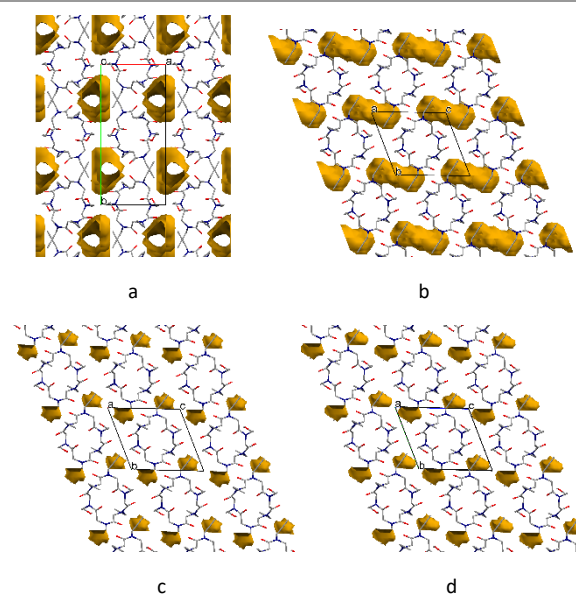
Fig. 3 Contact surfaces (yellow) in the crystal structures of 1 (probe radius: 1.2 Å). a) Form 1A : channels ( V = 196.2 Å 3 per unit cell) parallel to the c axis; b) form 1D : cavities ( V = 84.4 Å 3 ) stacked along the c axis; c) form 1E : cavities ( V = 11.9 Å 3 ) stacked along the c axis; d) form 1F : cavities stacked along the c axis ( V = 14.6 Å 3 ).
