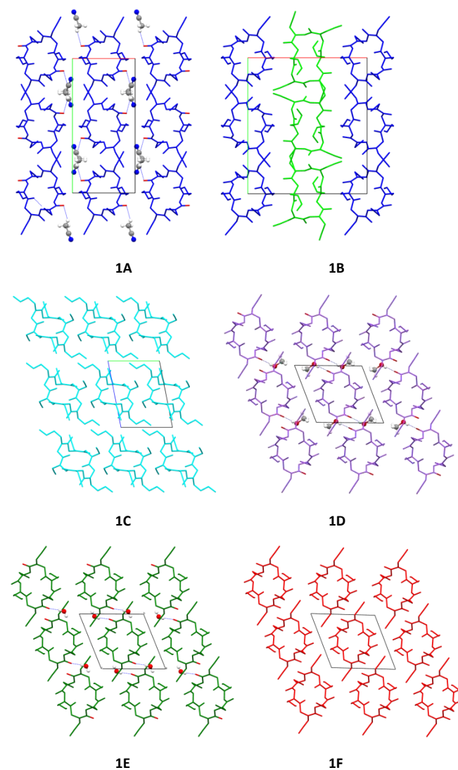
Fig. 2 Crystal packing of crystal forms 1A , 1B (type I molecules in blue; type II molecules in green), 1C , 1D , 1E and 1F as viewed along the shortest crystallographic axis. Host binding sites are highlighted in red. Guest molecules are depicted as ball and stick. Hydrogen atoms are visualized only for guest molecules.
