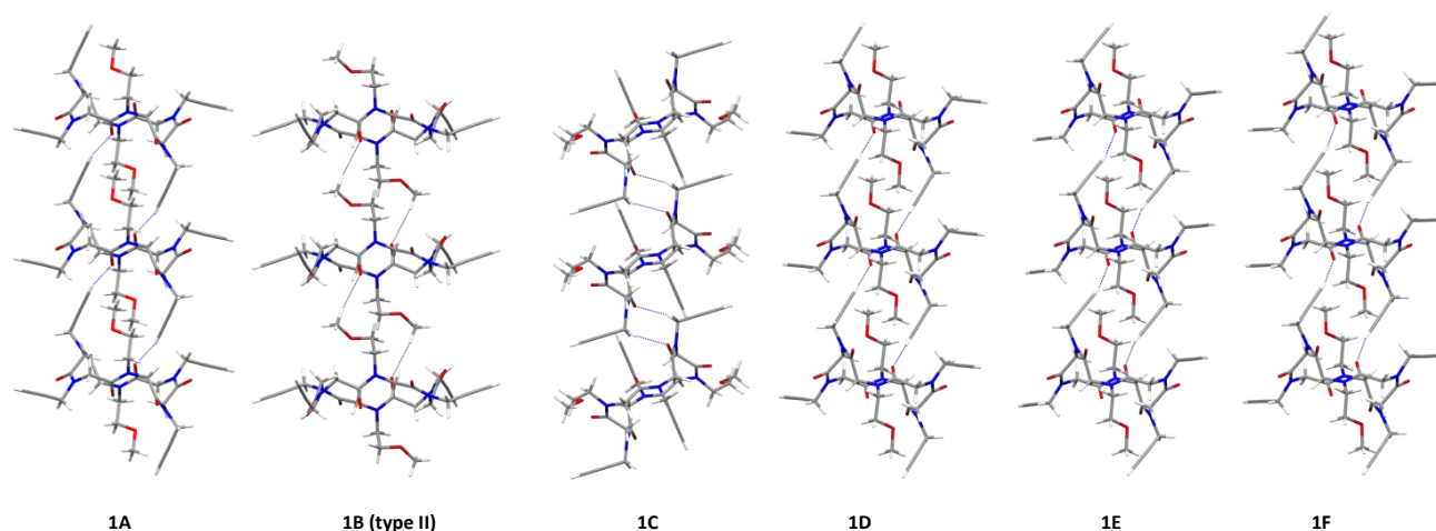
Fig. 1 Arrangement of cyclopeptoid molecules along the shortest crystallographic axis in crystal forms 1A , 1B type II molecules, 1C , 1D , 1E and 1F . C=O...H-C hydrogen bonds are depicted as dotted lines. Atom types: C grey, N blue, O red, H white.
