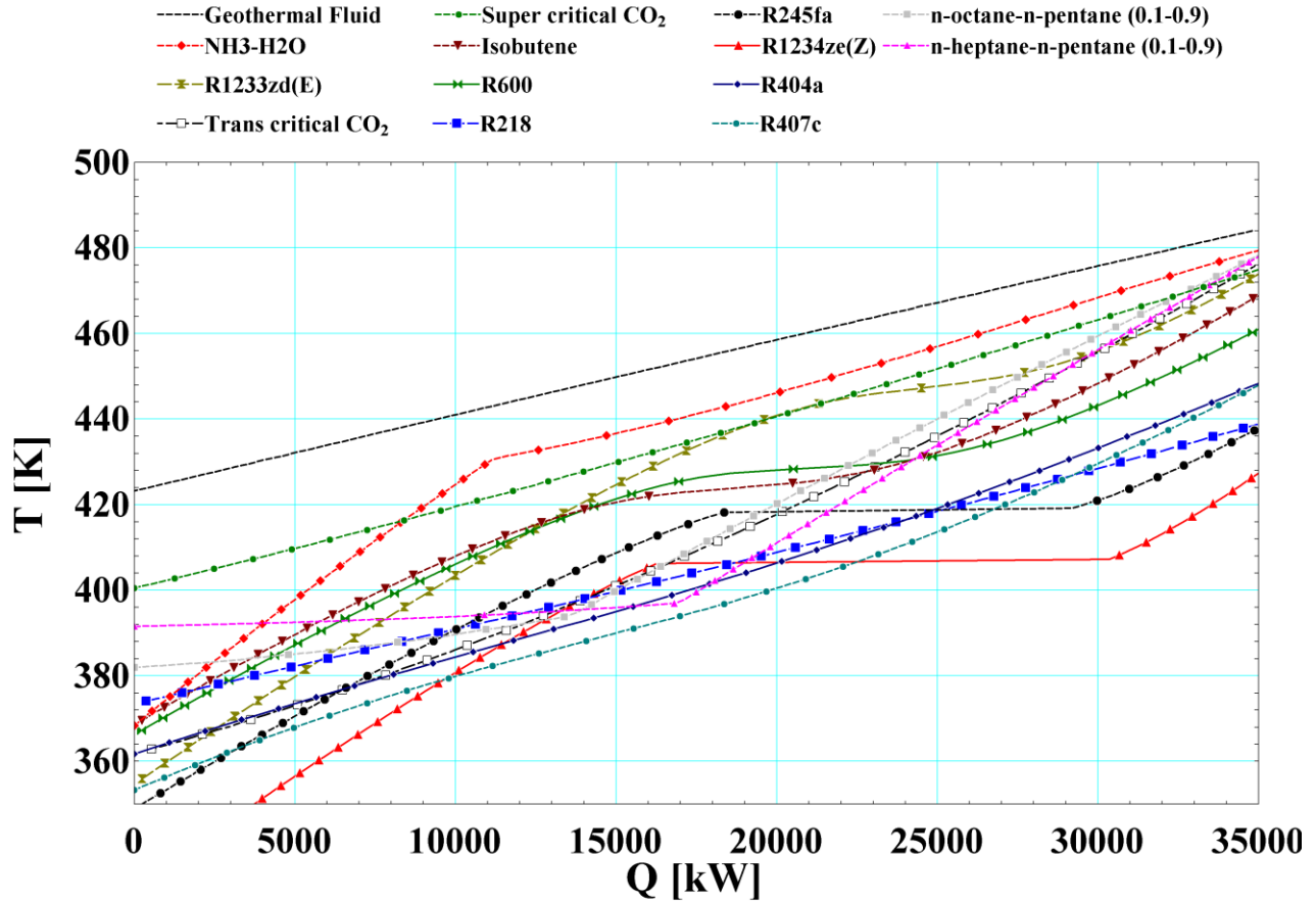
Figure 7 Comparison of heat transfer temperature profiles inside the evaporator, for the Mt. Amiata case study. The dashed black line represents the cooling curve of the geothermal fluid.
