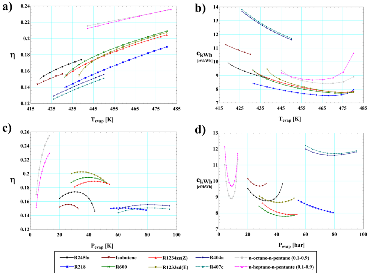
Figure 5 ORC efficiency and produced energy unit cost as a function of Evaporator temperature (a-b) and pressure (c-d)
