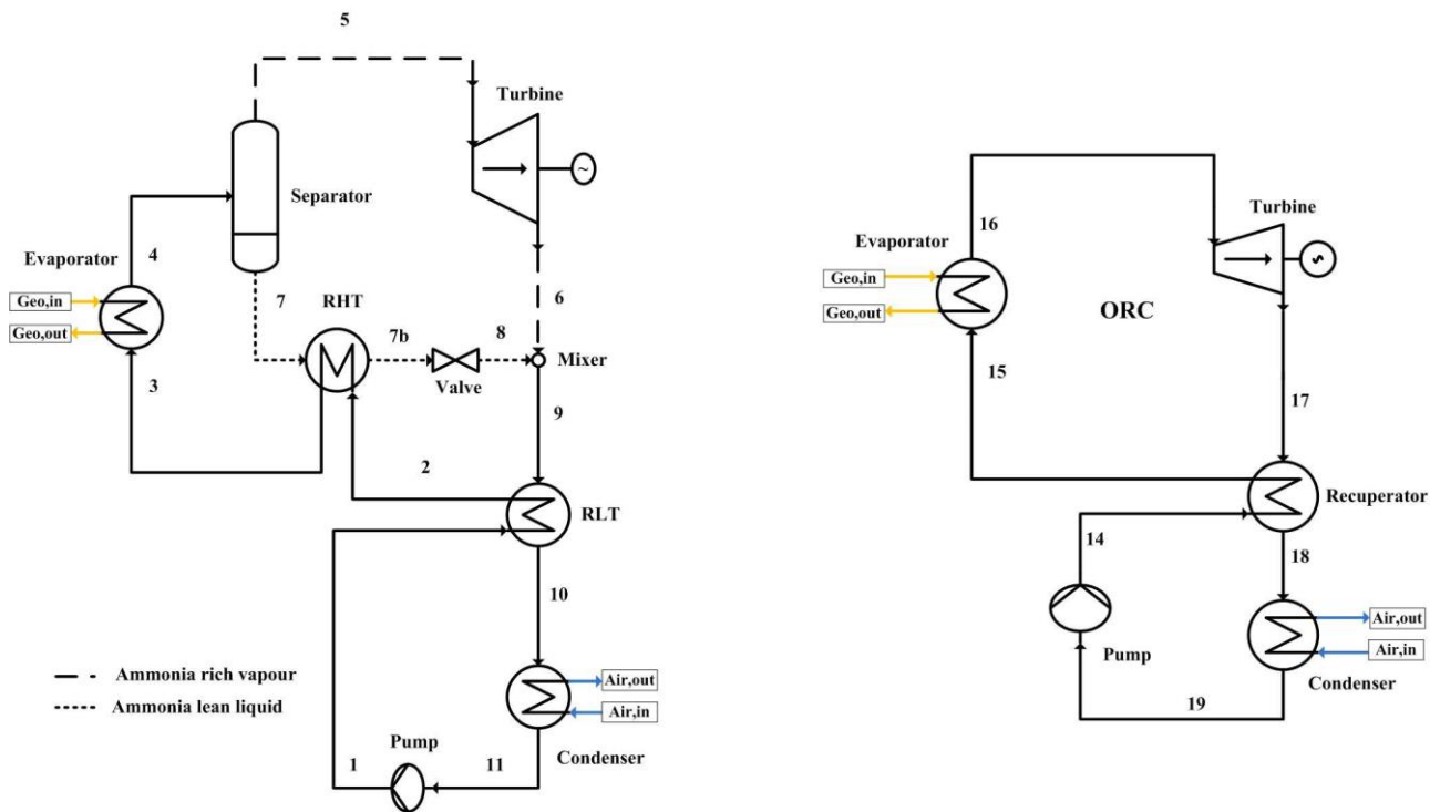
Figure 1 Schematic of KC (left side) and ORC cycle (right side)
