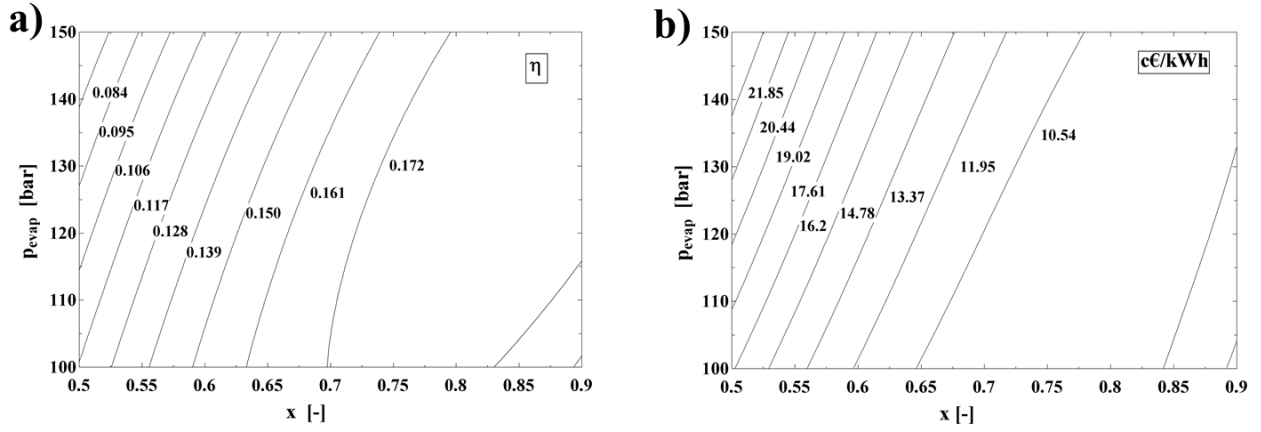
Figure 4 Contours of Thermal efficiency (a) and produced energy unit cost (b, [c€/kWh]) for KC, vs. evaporator pressure and ammonia mass fraction. Evaporator Temperature = 480 K; Condenser pressure = 9 bar
