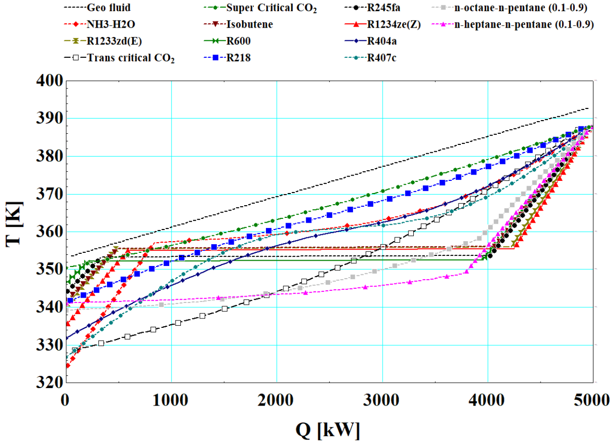
Figure 9 Thermal profiles comparison inside the evaporator, for the Pomarance case study. The dashed black line represents the cooling curve of the geothermal fluid
