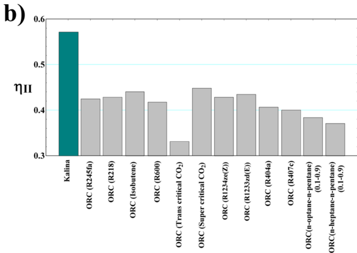
Figure 10a) Comparison of components relative exergy destructions between KC and ORCs; b) Second law efficiency comparison between KC and ORCs
