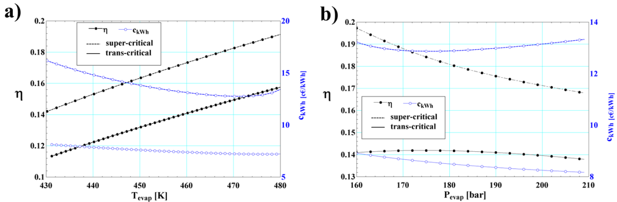
Figure 6 Efficiency and produced energy unit cost for the ORC Cycle, as a function of the maximum temperature (a) and the higher pressure level (b) of the cycle. ORC Working Fluid = Carbon Dioxide
