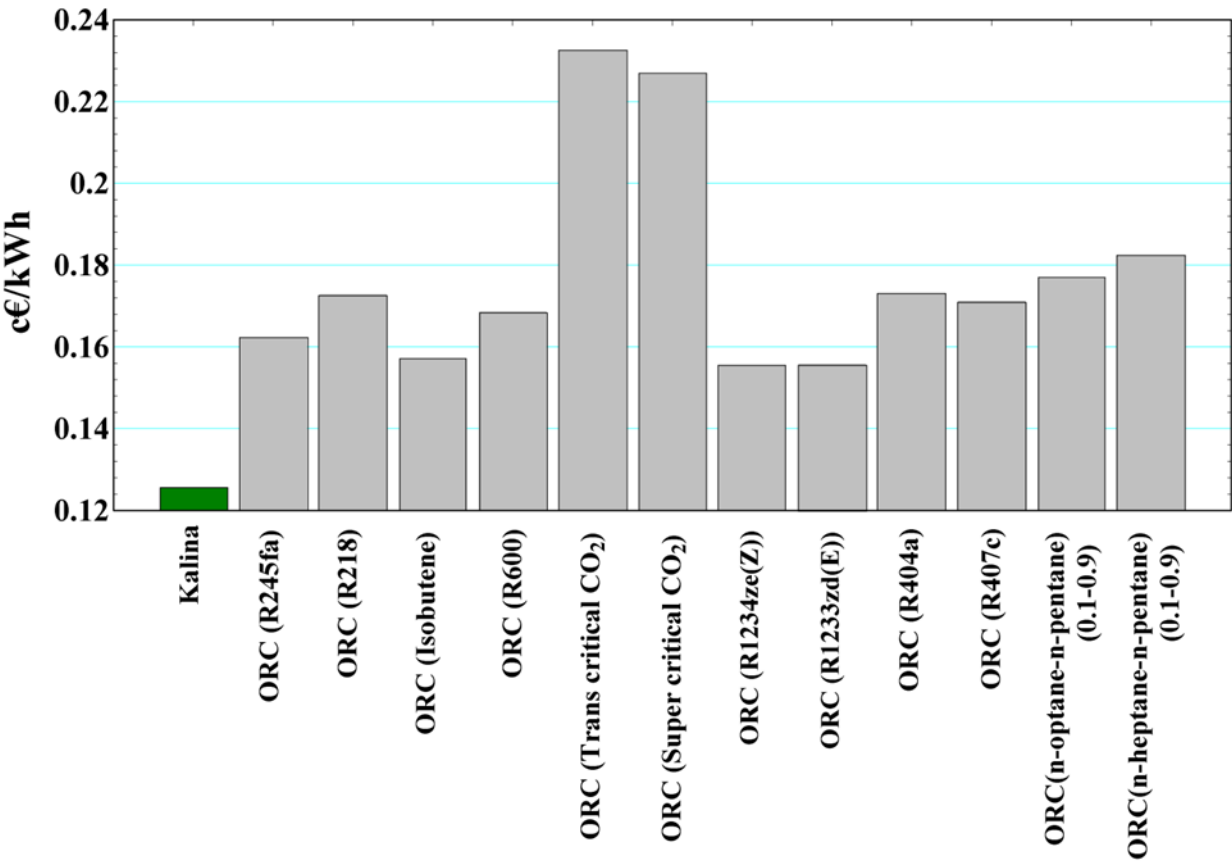
395 396 Figure 12 Comparison of electricity costs for the analysed power plants, Pomarance case study
