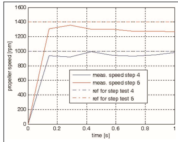
Figure 30. Results of step tests 4 and 5 (sampling/acquisition frequency of 0.144 ms).
