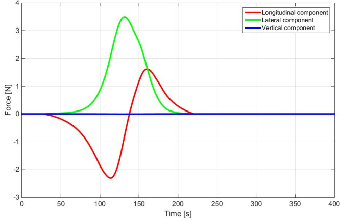
Figure 25: Vehicle 1: force due to the V^{v-e} potential related to the first obstacle
