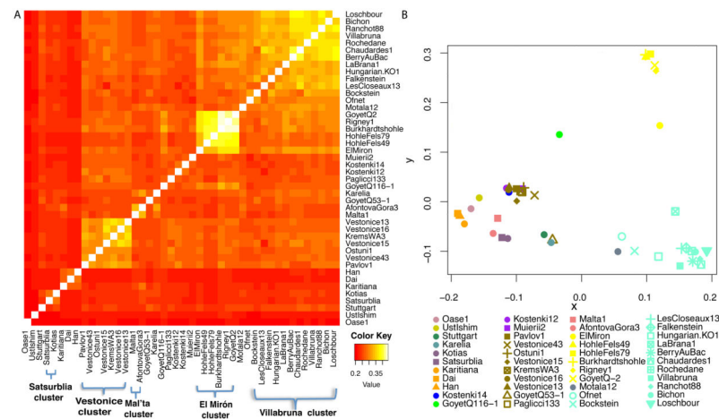
Figure 3. Genetic clustering
