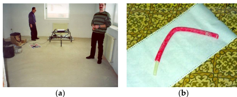
Figure 22. (a) MiRascan radar at work and (b) sample of plastic tubing.
