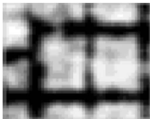
Figure 8. Radar image of reinforcing in concrete at 3.9 GHz. Mesh spacing is 20 cm \times 20 cm at a depth of 3 cm to 4 cm [39].
