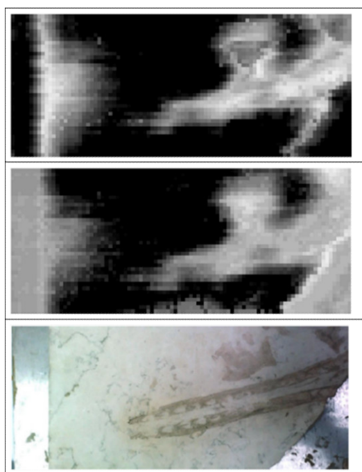
Figure 35. Summed modulus of parallel and cross-polarization scans at 6.7 GHz (top); summed modulus of scans 6.4 GHz, 6.5 GHz, 6.6 GHz, and 6.7 GHz parallel and cross-polarization (middle); and photograph of the lower side of the limestone slab aligned to correspond with the scanned area (bottom).
