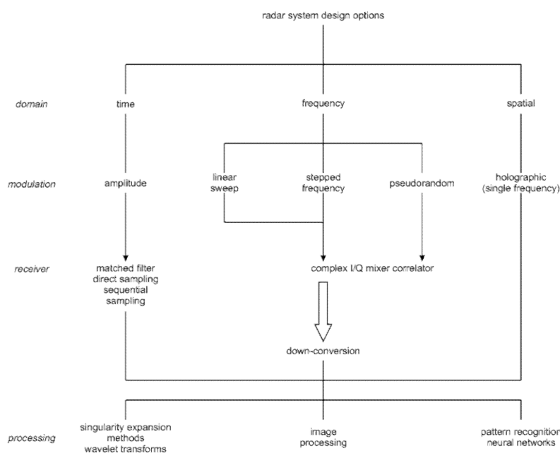
Figure 1. Classification of main types of subsurface radar [2].
