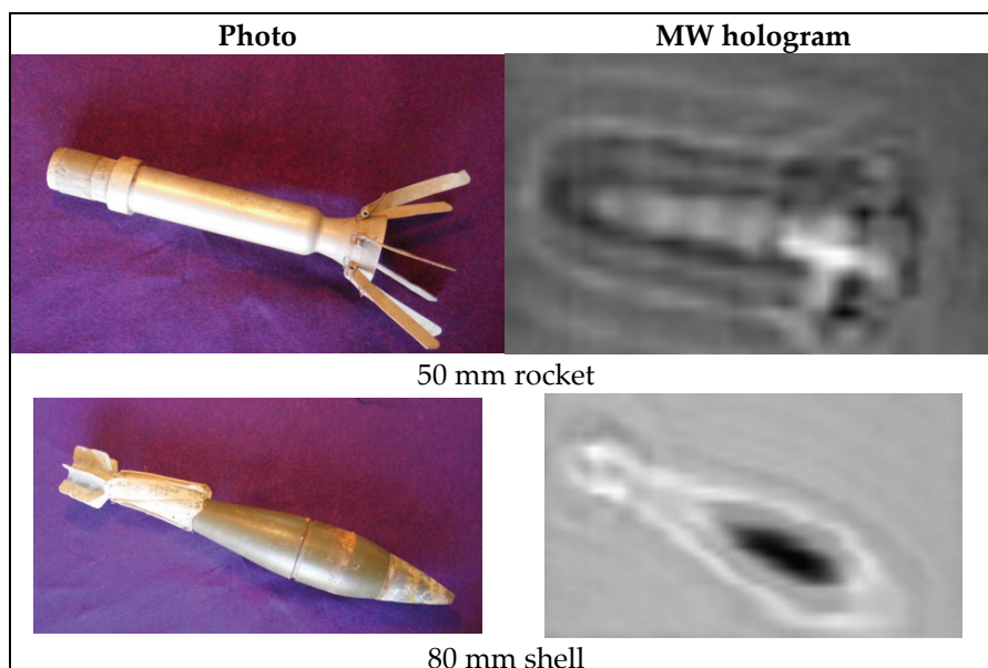
Figure 17. HSR images recorded by RASCAN-4/4000.
