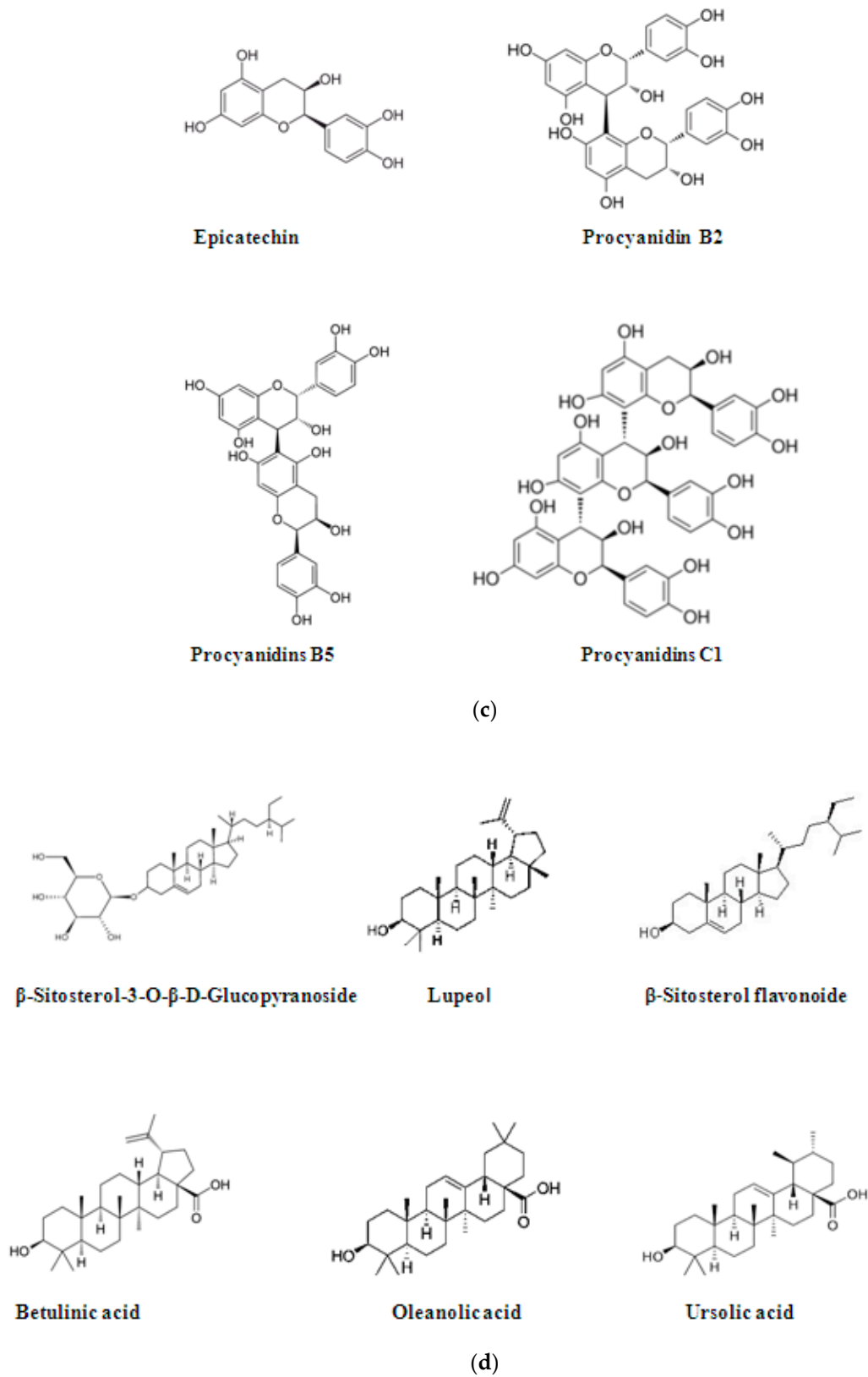
Figure 2. Chemical structure of acids quantified in C. monogyna fruits, plants and flowers. (a) Phenolic acids; (b) flavonoids and glycosylates derivatives in C. monogyna fruits, plants and flowers; (c) other flavonoids: epicatechin and procyanidin; (d) triterpenoid compounds.
