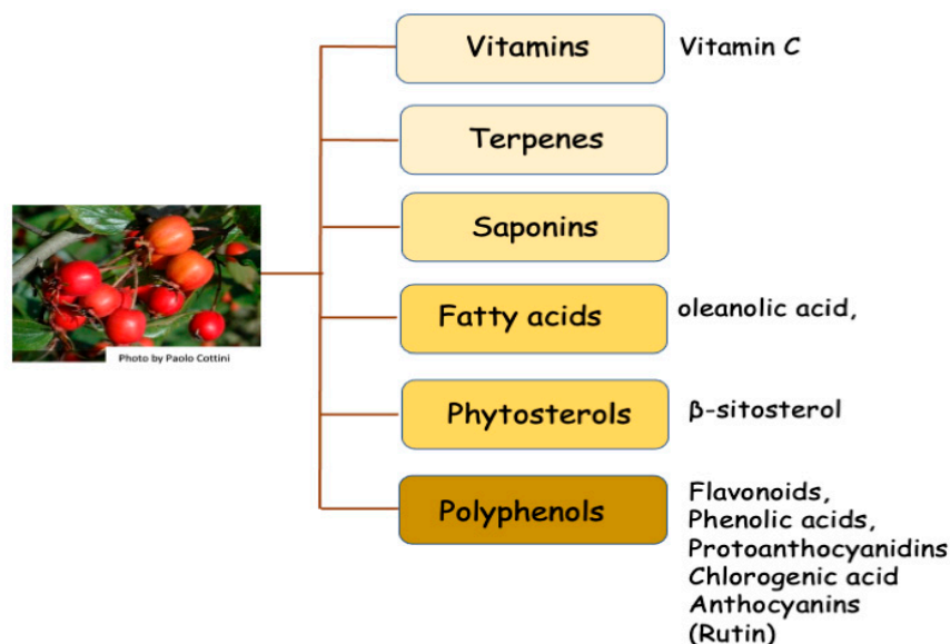
Figure 1. The main phytochemical components of C. monogyna are divided into different principal classes.
