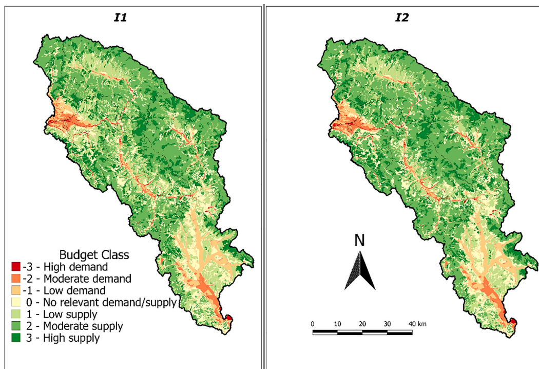
Fig. 8. ES budget maps obtained with the two indicators for the year 1990.
