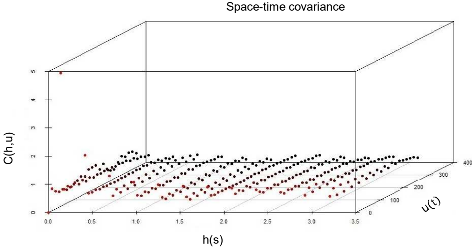
Figure 2. Sample covariogram.
