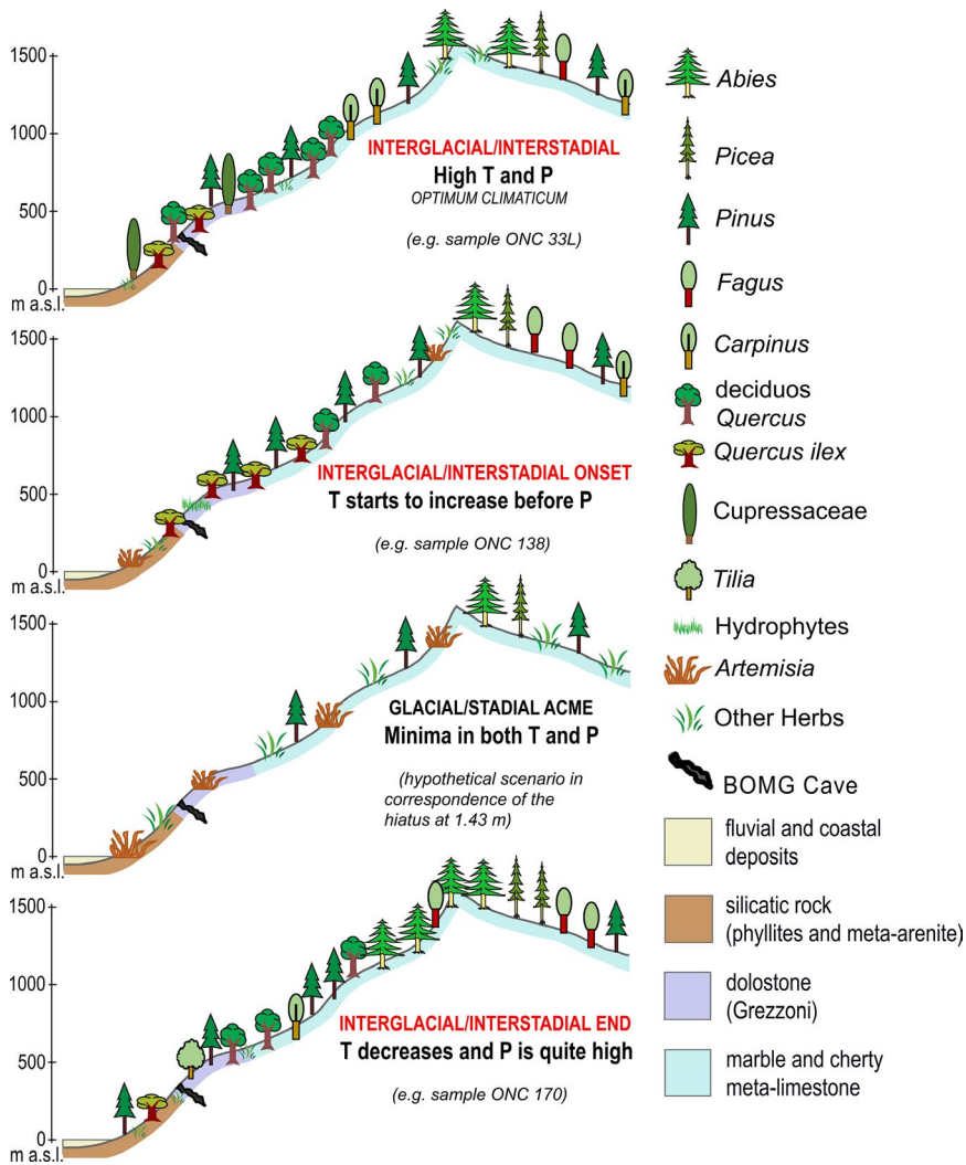
FIGURE 9 Schematic reconstruction summarising the dominant vegetation phases within the BOMG flowstone assuming that it formed from the Middle Pleistocene. The altitudinal profile ideally represents the morphology during flowstone deposition
