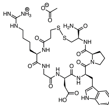
Figure 1. Eptifibatide acetate: N^6 -(aminoiminomethyl)- N^2 -(3-mercapto-1-oxopropyl)-L-lysylglycyl-L- \alpha -aspartyl-L-tryptophyl-L-prolyl-L-cysteinamide, cyclic (1→6)-disulfide acetate.
