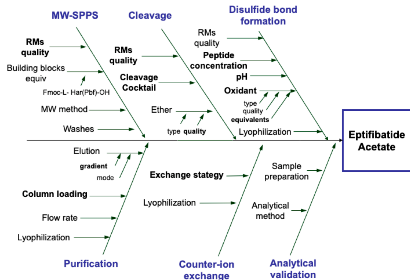
Figure 2. Ishikawa diagram for the development of the cGMP eptifibatide acetate production process. Critical process parameters (CPPs) are reported in bold.
