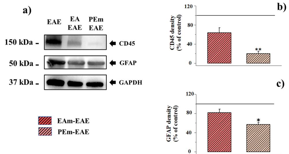
Figure 9. Effect of “in vivo” EAm and PEm treatments on the content of CD45 and of the glial fibrillar astrocytic protein (GFAP) in EAE mouse spinal-cord homogenates. (a) Representative Western blot of the immunostainings for CD45, GFAP and glyceraldehyde-3-phosphate dehydrogenase (GAPDH) in untreated, EAm-treated and PEm-treated EAE mouse spinal-cord homogenates. The protein GAPDH was used as the internal control. The blot is representative of the analysis on lysates from 6 animals for each experimental group. (b) Quantification of the change of CD45 density in the spinal-cord homogenates of EAm-treated ( n = 6 mice) and PEm-treated ( n = 6 mice) EAE mice versus the untreated ones ( n = 6 ). Results are calculated as CD45 \div GAPDH ratio and are expressed as percentage of the respective ratio in untreated EAE mice ( 1.12 \pm 0.22 ). Data are expressed as mean \pm SEM. (c). Quantification of the change of GFAP density in the spinal cord homogenates of EAm-treated ( n = 6 mice) and PEm-treated ( n = 6 mice) EAE mice versus that of untreated ones ( n = 6 ). Results are calculated as GFAP \div GAPDH ratio and are expressed as percentage of the respective ratio in untreated EAE mice ( 3.52 \pm 0.41 ). Data are expressed as mean \pm SEM. Note: * p < 0.05 versus untreated EAE mice; ** p < 0.01 versus untreated EAE mice. EA and PEm administration did not cause significant changes in the expression of the CD45 and the GFAP protein densities in control mice.
