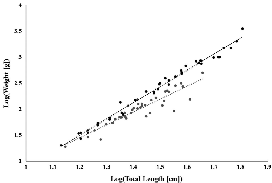
FIGURE 2 Log-transformed length-weight relationship of Ictalurus punctatus (black; y = 3.1177x - 2.2405 ; R^2 = 0.9874 ) and Silurus glanis (grey; y = 2.4836x - 1.5297 ; R^2 = 0.84 )
