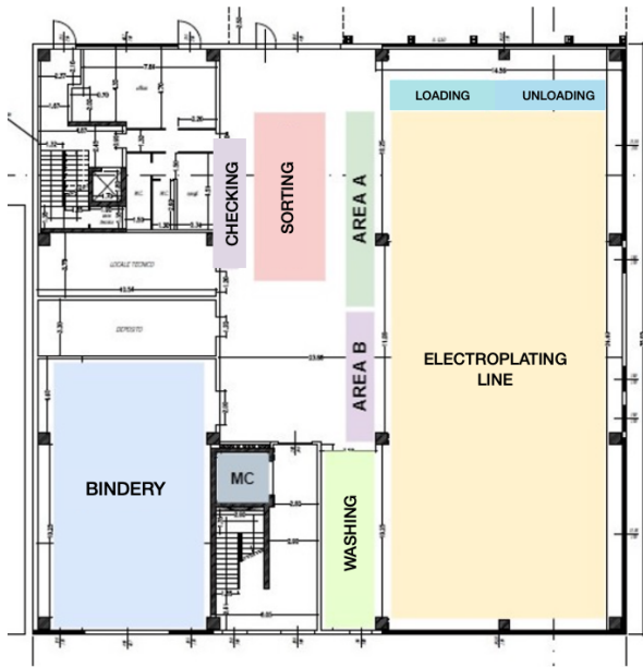
Figure 1: Plant layout
