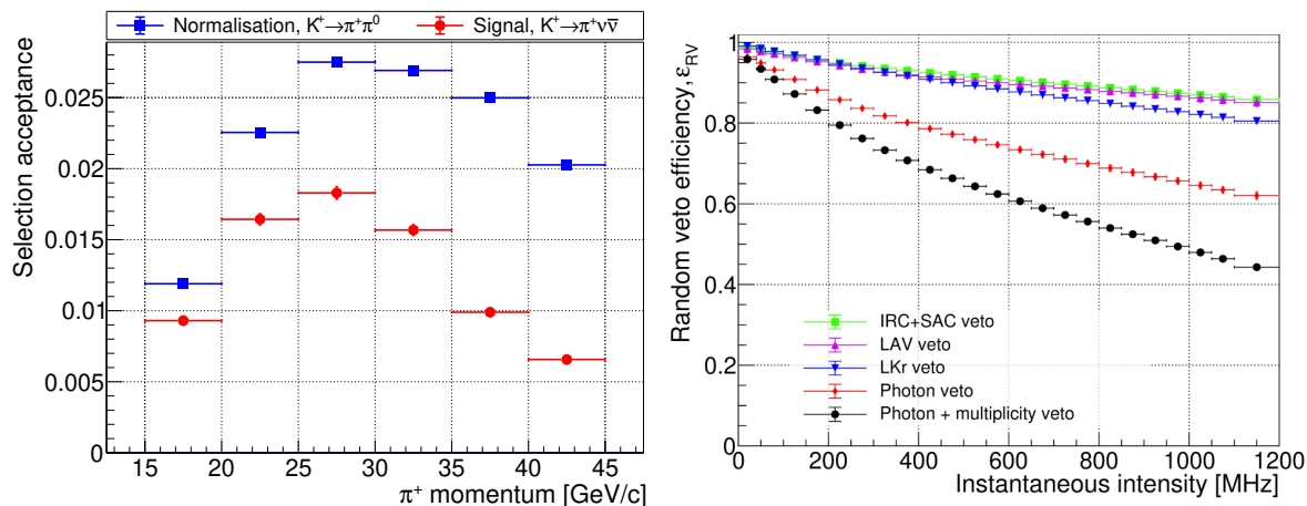
Figure 4. Left: selection acceptances, A_{\pi\pi} and A_{\pi\nu\bar{\nu}} , as functions of \pi^+ candidate momentum displayed as blue squares and red circles, respectively. Right: random veto efficiency as a function of the instantaneous beam intensity.
