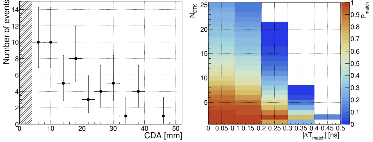
Figure 9. Left: distribution of the CDA variable for events in the upstream reference sample (URS). Right: matching probability P_{\text{match}} measured in the K^+ \rightarrow \pi^+ \pi^0 normalisation sample in bins of \Delta T_{\text{match}} and N_{\text{GTK}} .
