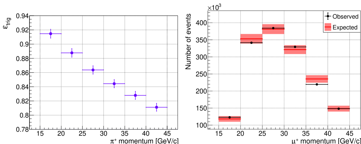
Figure 5. Left: trigger efficiency ratio \epsilon_{\text{trig}} as a function of the of \pi^+ momentum. Right: expected and observed numbers of K^+ \rightarrow \mu^+\nu events in trigger efficiency validation samples, as a function of the \mu^+ momentum.
