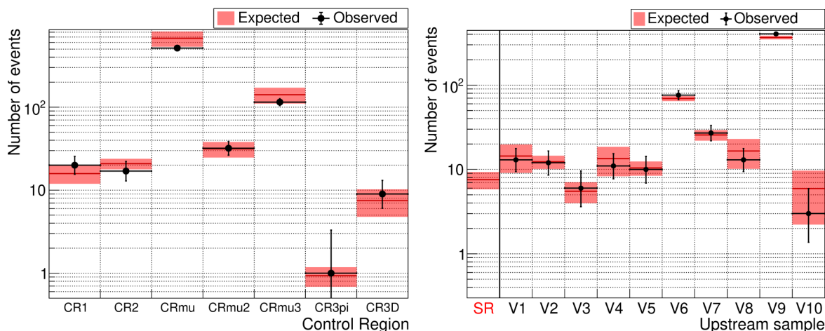
Figure 8. Left: expected and observed numbers of events in the control regions shown in figure 3-right. The global p -value of the comparison is 0.80, the lowest single-region p -value is 0.24. Right: expected and observed numbers of events in the upstream validation samples. The first bin is the signal region and therefore only the expectation is displayed. The global p -value is 0.97, the lowest single-sample p -value is 0.14.
