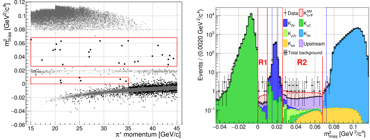
Figure 10. Left: distribution of the observed data events satisfying the signal selection criteria in the (p_{\pi^+}, m_{\text{miss}}^2) plane. Events in the background, control and signal regions are shown by small grey, small black and large black markers, respectively. Right: m_{\text{miss}}^2 projection including SM signal [1] (assuming \mathcal{B}_{\pi\nu\bar{\nu}}^{\text{SM}} = 8.4 \times 10^{-11} ) and background expectations from K^+ \rightarrow \pi^+\pi^0 ( K_{2\pi} ), K^+ \rightarrow \mu^+\nu ( K_{\mu 2} ), K^+ \rightarrow \mu^+\nu\gamma ( K_{\mu 2\gamma} ), K^+ \rightarrow \pi^+\pi^+\pi^- ( K_{3\pi} ), K^+ \rightarrow \pi^+\pi^-e^+\nu ( K_{e4} ) and upstream. The total expected background and its uncertainty is shown by the black line and hatched bars, respectively. In the signal region R1, events in the momentum range 35–45 GeV/ c are excluded.
