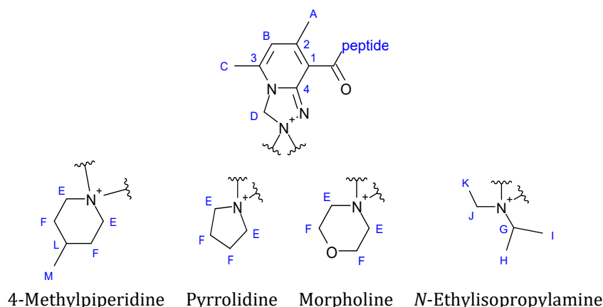
Figure 28. Signed atoms in 5,7-dimethyl-2,3-dihydro[1,2,4]triazolo[4,3- a ]pyridine-8-carboxylic acid derivatives, for the purpose of NMR chemical shifts assignment. Proton groups are signed with letters (A-M); carbons with numbers (1-4).
