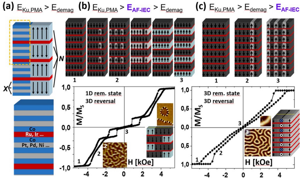
Figure 12. (a) PMA-SAFs ( E_{Ku,PMA} > E_{demag} ) based on double multilayer (X, N) magnetic meta-materials, architecture (top), respective material options (bottom). (b), (c) Typical magnetic field reversal for (b) E_{Ku,PMA} > E_{AF-IEC} > E_{demag} . Reproduced from [73]. CC BY 4.0, and (c) E_{Ku,PMA} > E_{demag} > E_{AF-IEC} . Reproduced from [80]. CC BY 4.0. The top displays schematic illustrations of the reversal from negative saturation to remanence. The bottom shows respective VSM hysteresis loops. Specific reversal stages are labeled for better cross-comparison. Top-down MFM domain images ( 2\ \mu\text{m} \times 2\ \mu\text{m} each) are added as insets for reversal state 2 in (b) and for the remanent state 3 in (c) together with a schematic cross-sectional domain wall image. While for case (b) the remanent state is still 1D AFC, for (c) it becomes a complex 3D mixed FM/AF domain structure. The two bottom right insets in (b) display an MFM image together with a cross-sectional scheme of a metastable AF antiphase domain state separated by a 1D FM stripe domain phase as obtained after out-of-plane AC demagnetization.
