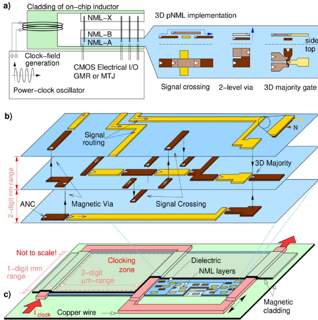
Figure 30. (a) Nanomagnetic digital gates are stacked in the end-of-line technology of CMOS chips and powered/synchronized by a magnetic field. (b) Ion-beam engineering to control domain reversal and domain-wall motion for signal routing is applied in a 3D stack. (c) A highly permeable cladding combined with meander-like copper wires provides the magnetic field-clock. Reprinted from [185], Copyright (2016), with permission from Elsevier.
