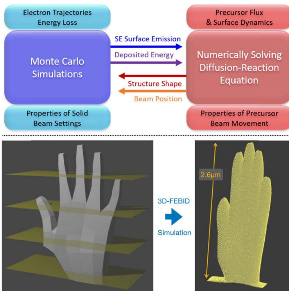
Figure 4. (top) Schematic of simulation process flow for 3D-FEBID using reaction-diffusion equation and Monte Carlo simulation. (bottom) 3D test model with exemplary slicing planes as indicated (left). Result of 3D-FEBID simulation using the precursor \text{Me}_3\text{CpMePt} (right).
