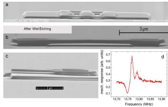
Figure 7. (a) A ‘trampoline’ YIG resonator where a large free-standing mass is coupled by thin connectors to the posts on the substrate. (b) YIG bridge optimized by wet etching for extremely smooth surfaces and edges. (c) YIG cantilever and (d) mechanical resonance of the cantilever measured by interferometry. The quality factor is >500 .
