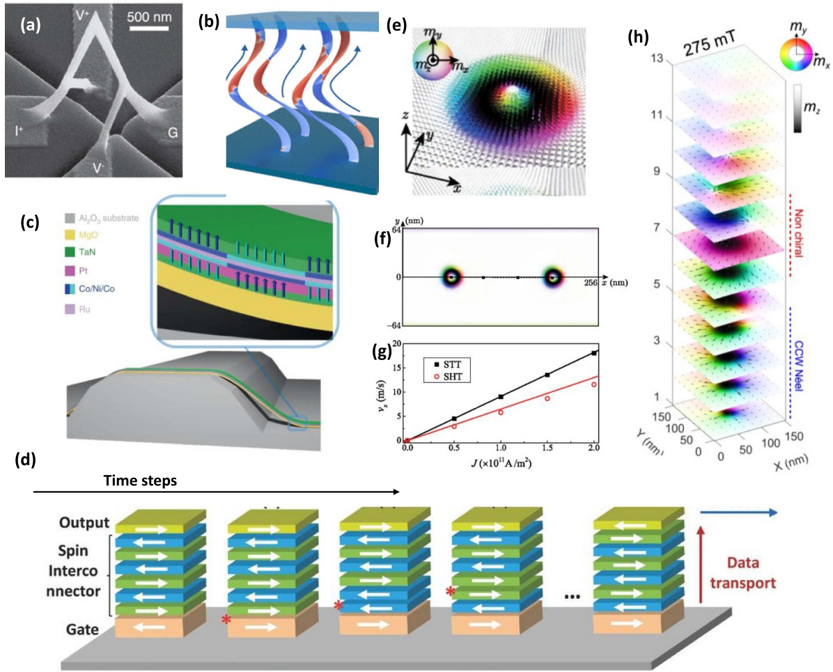
Figure 34. Recent works related to 3D spintronic devices. (a) Ferromagnetic interconnector directly printed by FEBID. Reproduced from [10]. CC BY 4.0. (b) Automation of magnetic bits in between planes using interconnectors with in-built gradients. Reproduced from [145]. CC BY 4.0. (c) State-of-the-art racetrack memories formed by synthetic antiferromagnets, positioned on 3D pre-patterned substrates to achieve vertical domain wall motion. Reproduced from [11]. CC BY 4.0. (d) Concept for MRAM with vertical magnetic bit transfer functionality. Reproduced from [202]. CC BY 4.0. (e)–(g) Theoretical study of current-induced motion of a Hopfion in a racetrack device. Reprinted (figure) with permission from [203], Copyright (2019) by the American Physical Society. (h) Micromagnetic simulations of a skyrmion cocoon formed along the height of ultra-thin magnetic multilayers, obtained by engineering the heterostructure energies. Reproduced from [113]. CC BY 4.0.
