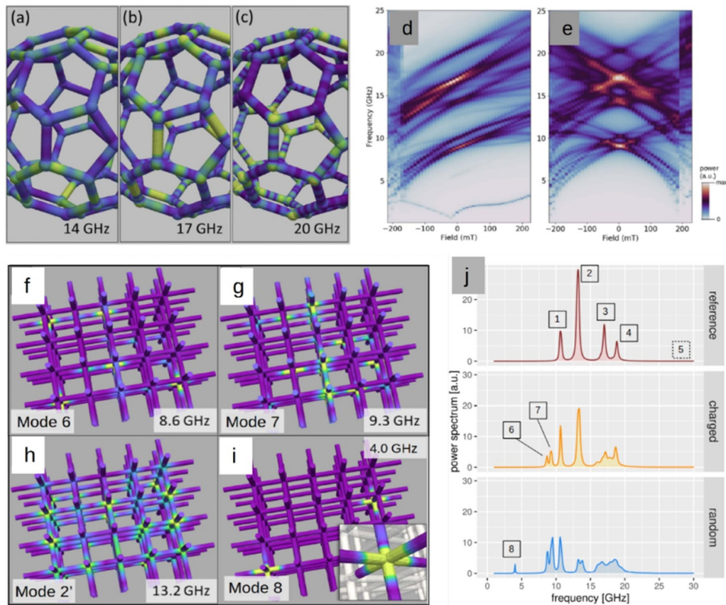
Figure 26. Advanced simulation methods in the frequency domain make it possible to conduct systematic simulations on the high-frequency magnetization dynamics, like spatial configuration and field dependence of resonance spectra for different magnetic oscillations in a buckyball geometry (see panels (a)–(e) reproduced from [170]. CC BY 4.0.) and to address the configuration dependence of the oscillatory dynamics in larger arrays of interconnected nanowires (see panels (f)–(j) reproduced with permission from [166]).
