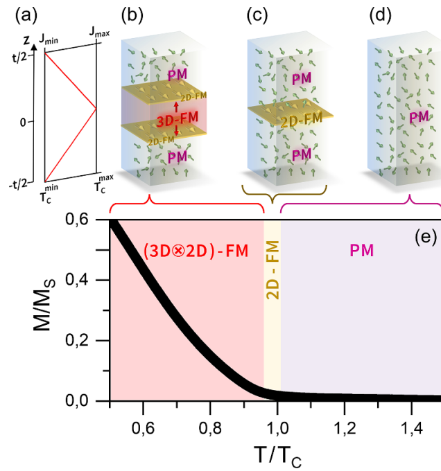
Figure 13. (a) Schematics of the exchange coupling depth profile and (b)–(d) of the magnetic state profiles upon changing the temperature of a single crystal CoRu alloy film. (e) Corresponding temperature dependence of the normalized magnetization.
