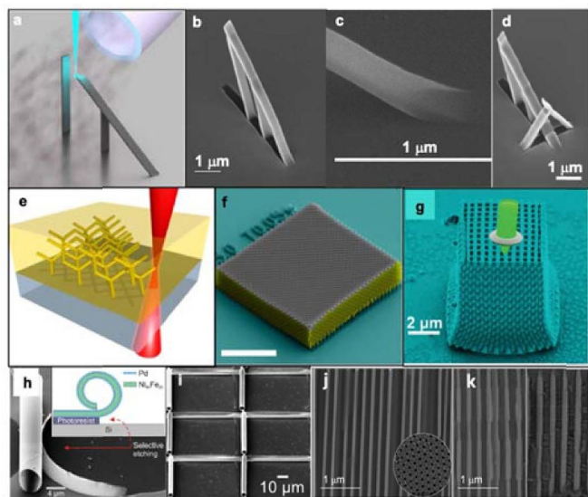
Figure 2. Overview of fabrication methodologies used to realise 3D magnetic nanostructures. (a) Focussed electron beam induced deposition, which has been used to realise (b)–(d) tilted 3D magnetic nanowires for domain wall injection [22]. Reproduced from [22]. CC BY 4.0. (e) Two-photon lithography which has been used to realise a range of structures including (f) a 3D artificial spin-ice [2]. Reproduced from [2]. CC BY 4.0. (g) a 3D nanomagnetic network [23]. Reproduced from [23]. CC BY 4.0. (h) Rolled-up ferromagnetic microtubes [24]. (i) Microtubes in a patterned array [24]. Reproduced from [24]. © IOP Publishing Ltd All rights reserved. (j), (k) FeCo nanowires with uniform and modulated diameters fabricated by electrodeposition into alumina templates (inset) [25]. Reproduced from [25]. CC BY 4.0.
