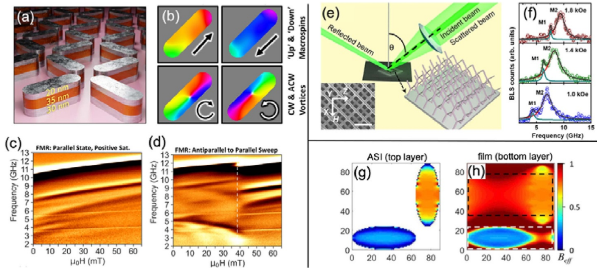
Figure 15. (a)–(d) Demonstration of ultrastrong magnon-magnon coupling and chiral symmetry breaking in a 3D layered artificial spin ice (ASI): (a) Schematic illustration of array. (b) Four possible macrospin and vortex nanoisland magnetization states. (c) Parallel state exhibiting only the acoustic magnon mode, whereas (d) antiparallel state also shows the optical magnon mode. (c), (d) Reproduced from [93]. CC BY 4.0. (e), (f) Coherent spin waves in a 3D ASI detected by Brillouin light scattering (BLS): (e) Schematic of measurement configuration with scanning electron microscope image as inset. (f) Various magnon modes detected by BLS. (e), (f) Reproduced from [92]. CC BY 4.0. (g), (h) Observation of dynamic coupling in a magnetic hybrid system made of an artificial spin-ice structure and an extended NiFe underlayer: ASI mode in the top ASI layer (g) imprints dynamics in the thin film underlayer (h). (g), (h) Reproduced from [91]. CC BY 4.0.
