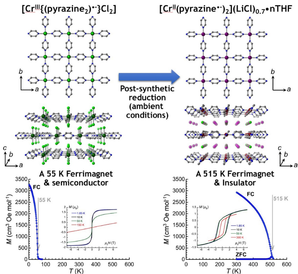
Figure 20. Scheme illustrating the post-synthetic reduction of the pre-formed [\text{Cr}^{\text{III}}\{(\text{pyrazine}_2)^{\bullet\bullet}\}\text{Cl}_2] pyrazine-based coordination network to form the 515 K ferrimagnet, [\text{Cr}^{\text{II}}(\text{pyrazine}^{\bullet\bullet})_2](\text{LiCl})_{0.7}\cdot n\text{THF} . Their associated magnetic properties (as M vs T and M vs H plots) are also shown on the lower part of the figure. Colour code: C, grey; N, blue; \text{Cr}^{\text{III}} , dark green; \text{Cr}^{\text{II}} , dark purple; Cl, light green; Li, purple. Adapted from references [124, 125].
