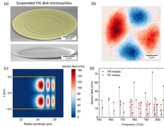
Figure 6. (a) Two suspended YIG disk microcavities, one with a ‘disk on a stem’ structure (diameter of 50 \mu\text{m} ) and one with a suspended edge structure (diameter of 25 \mu\text{m} ). The YIG disks are 150 nm thick, and their edge is lifted \sim 1 \mu\text{m} above the GGG substrate. (b) Super Nyquist-sampling magneto-optical Kerr effect (SNS-MOKE) image of a radially symmetric magnon mode in a suspended YIG disk microcavity with a diameter of 7.5 \mu\text{m} . (c) COMSOL simulation of the electric field distribution of a WGM mode in a YIG disk microcavity. (d) WGM spectrum for TM and TE polarized modes in the same cavity.
