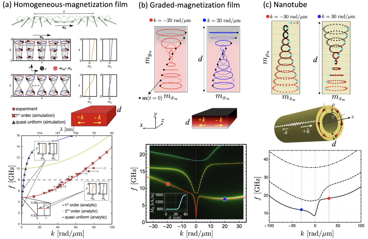
Figure 23. Spin-wave dispersion and magnetization profiles across the thickness of (a) homogeneous-magnetized film, (b) graded-magnetized film, and (c) nanotube. In (a) and (b) the equilibrium magnetization is in plane, while in (c) a vortex ground state is assumed. In all cases a breakdown of the usual quantization condition is observed. (a) Reprinted (figure) with permission from [156], Copyright (2019) by the American Physical Society. (b) Reproduced from [154]. © IOP Publishing Ltd CC BY 3.0. (c) Reprinted (figure) with permission from [160], Copyright (2022) by the American Physical Society.
