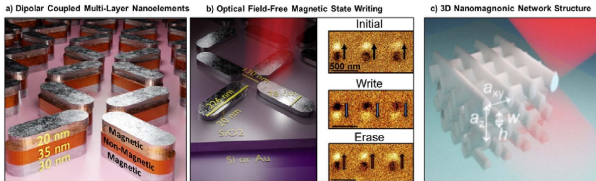
Figure 31. 3D nanomagnetic systems and field-free writing approaching. (a) Multilayered systems comprising strongly dipolar-coupled magnetic nanoelements may offer benefits for 3D magnetic computing, allowing information exchange and physical interaction between discrete nanoelements via the intrinsic dipolar field, with both static and GHz dynamic components. This may be a route to reducing or avoiding huge amounts of electrical interconnects in 3D nanostructures. Reproduced from [187]. CC BY 4.0. (b) All-optical magnetic writing of nanostructures. 3D nanomagnetic systems require state control mechanisms that match the complexity of the 3D geometries if they are to be utilised as computing platforms. Mechanisms to write any nanomagnetic element, whether as a binary digital state or neuromorphic neuronal ‘weight’ are essential, particularly attractive if they avoid attaching electrical connections to every nanoelement. All-optical writing offers an appealing route forwards here, and has recently been demonstrated in 2D nanostructures. Reproduced with permission from [191]. CC BY-NC 4.0. (c) Promising examples of 3D nanomagnetic architectures which should be explored for neuromorphic computing schemes include densely connected nanowire networks such as the example here from reproduced from [23]. CC BY 4.0. Such systems offer both longer-range dipolar and strong short-range exchange coupling and the ability to host spin-waves/magnons which have been demonstrated as attractive potential information carriers in a host of 2D nanomagnetic neuromorphic computing schemes recently. The laser light here represents the two-photon lithography used to write the geometric structure, using such a voxel-focused laser with 3D spatial control could be an appealing future route towards 3D all-optical nanomagnetic writing similar to that shown in (b), albeit with technological challenges to be overcome.
