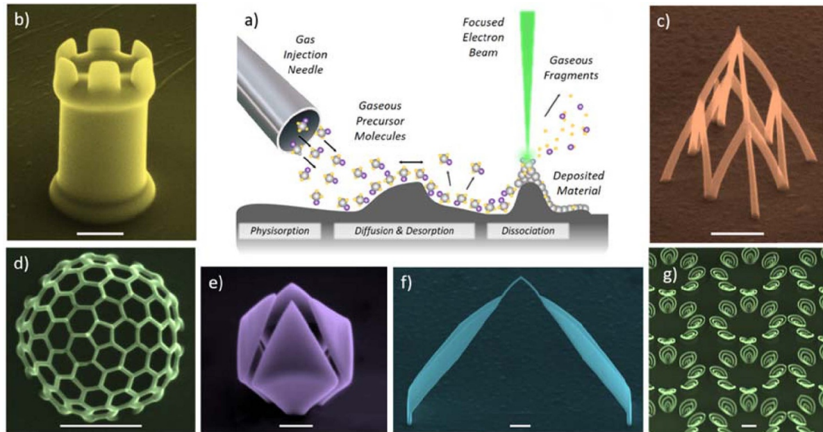
Figure 3. (a) Basic principle of FEBID, where a focused electron beam dissociates and immobilizes surface adsorbed precursor molecules. By the controlled beam movement, bulky (b) or mesh-like 3D structures (c) can be realized, allowing for more complex (d), sheet-like (e) and even combined (f) designs for fabrication of single objects (b)–(f) or larger arrays (g). All images are recolored, tilted SEM images with a 500 nm wide scale bar.
