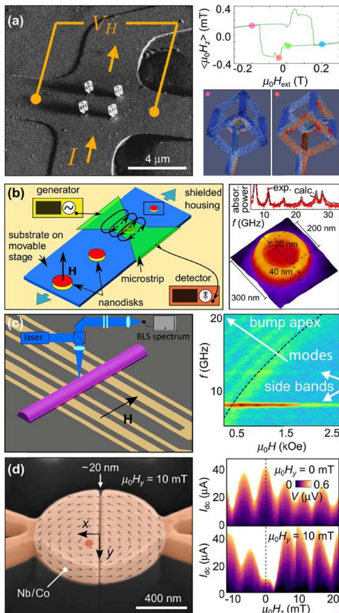
Figure 8. (a) SEM micrograph of a Hall cross with a 2 \times 2 array of nano-cubes on its surface in the Hall measurement configuration next to its numerically modeled magnetic hysteresis loop and magnetization configurations for the external magnetic field applied at an angle of 85^\circ relative to the surface normal of the Hall sensor. Reproduced from [52]. CC BY 4.0. (b) Left: Concept of spatially-resolved perpendicular spin-wave spectroscopy for a series of nanomagnets which are individually positioned close to a microwave excitation antenna. Reproduced from [55] with permission from the Royal Society of Chemistry. Right: Exemplary spin-wave eigenmode spectrum of a 3D Co-Fe nanovolcano in an out-of-plane magnetic field. The nonuniform internal field of the nanovolcano leads to a stronger confinement of the magnon eigenmodes within its crater. Reproduced from [53]. CC BY 4.0. (c) Schematic of a Co-Fe spin-wave conduit (plank with a bump along its axis) revealing a much richer BLS-FMR magnon spectra in comparison with a reference planar conduit. Reproduced from [54]. CC BY 4.0. (d) SEM image of a Josephson device (Nb/Co disk in which Nb electrodes are separated by a trench, forming a Co weak link) with the superimposed image of calculated spin texture for \mu_0 H_y = 10 mT. The vortex core (red dot) is shifted from the disk center and this affects the supercurrent interference pattern. Reproduced from [56]. CC BY 4.0.
