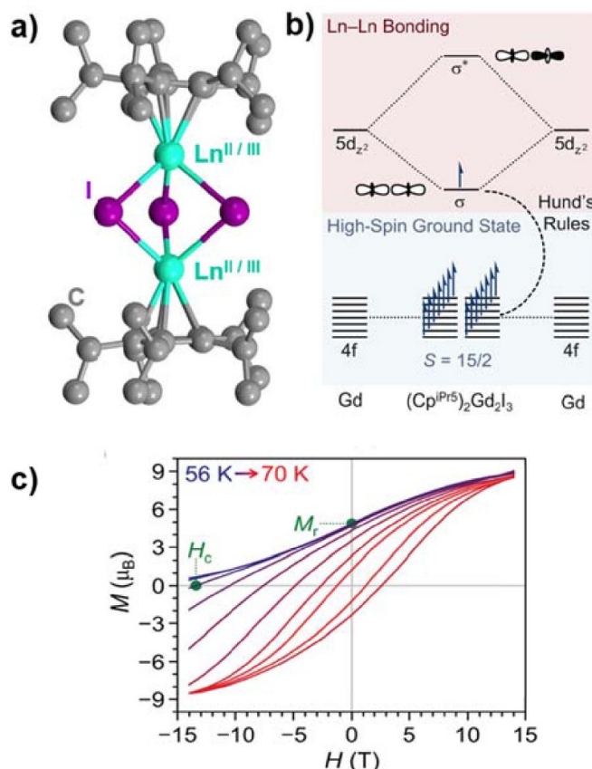
Figure 21. (a) Structure of the complexes of formula (\text{Cp}^{\text{iPr5}})_2\text{Ln}_2\text{I}_3 ( \text{Cp}^{\text{iPr5}} = penta-isopropylcyclopentadienyl; \text{Ln} = \text{Y}, \text{Gd}, \text{Tb}, \text{or Dy} ), (b) Molecular orbital diagram for (\text{Cp}^{\text{iPr5}})_2\text{Gd}_2\text{I}_3 illustrating the mechanism leading to strong ferromagnetic exchange interaction through the formation of a singly occupied \sigma -bonding orbital. (c) Temperature dependence of the magnetic hysteresis of the (\text{Cp}^{\text{iPr5}})_2\text{Dy}_2\text{I}_3 single-molecule magnet showing extremely hard magnetism. Adapted from Ref. [126]. Reprinted with permission from AAAS.
