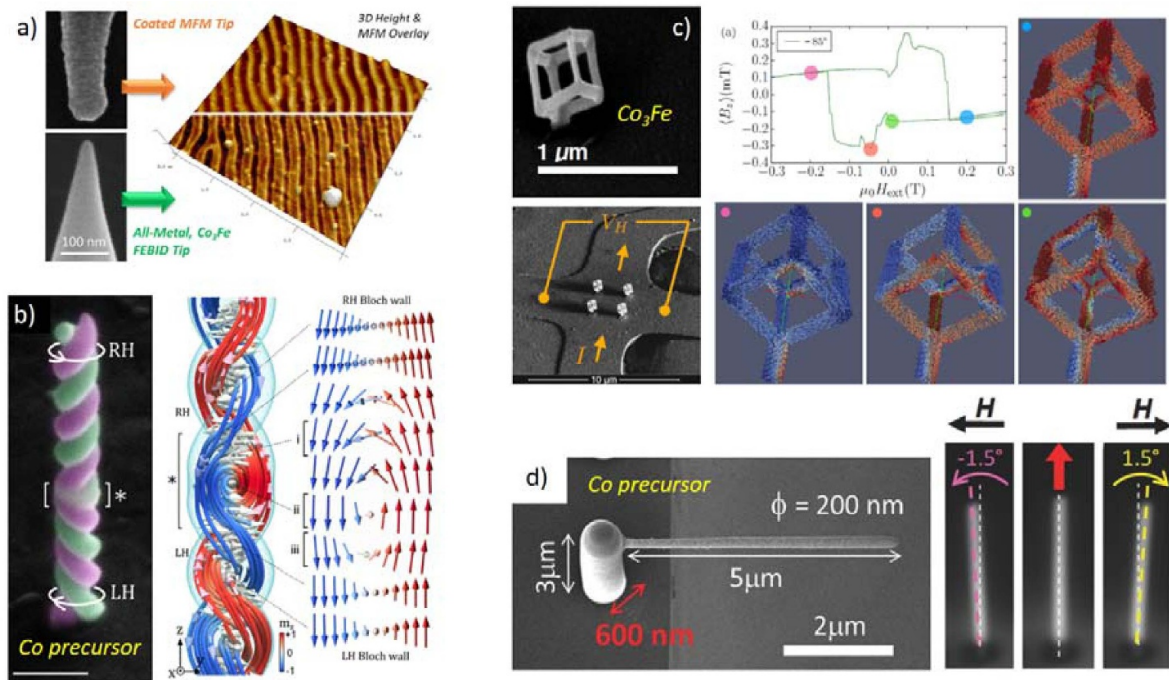
Figure 5. (a) SEM comparison of a commercial (top) and a 3D-FEBID (bottom) MFM nanoprobe. The associated MFM signals are shown on the right, illustrating the strongly improved performance due to the sharp all-metal character [36]. Reproduced from [36]. CC BY 4.0. (b) Colored SEM image of a close-packed Co double helix (left) with opposite chirality, complemented by micromagnetic simulations (center) revealing the opposite chirality with antiparallel magnetic alignment, as shown in more detail on the right by a RH to LH Bloch wall transition. Reproduced from [1]. CC BY 4.0. (c) Shows a complex \text{Co}_3\text{Fe} nano-cube (top) further placed on a micro-Hall sensor (bottom) that enables magnetic measurements, complemented by simulations to study the switching behavior of individual branches in response to the external field (right) [31]. Reproduced from [31]. CC BY 4.0. (d) Shows a composite nano-actuated magneto-mechanical system in a SEM top view (left), which bends left and right in response to an external magnetic field (right), therefore representing the basic element of a magneto-mechanical nanoactuator. [39] John Wiley & Sons. [Copyright © 2016 WILEY-VCH Verlag GmbH & Co. KGaA, Weinheim].
