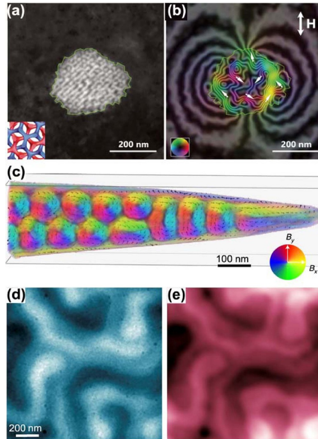
Figure 9. Phase contrast imaging with off-axis and in-line electron holography using aberration-corrected transmission electron microscopy. (a) Structure and (b) magnetic induction of 3D gyroid network visualized with off-axis holography. Reprinted with permission from [5]. Copyright (2020) American Chemical Society. (c) Magnetic induction of topological magnetic states in helimagnetic FeGe nano-cones obtained with holographic vector field electron tomography. Reproduced from [57]. CC BY 4.0. (d,e) Electron phase of ferrimagnetic domain walls in amorphous films with perpendicular magnetic anisotropy reconstructed with (d) iterative (Gerchberg-Saxton) and (e) non-iterative (transport-of-intensity) phase retrieval algorithms. Reproduced from [58], with permission from Springer Nature.
