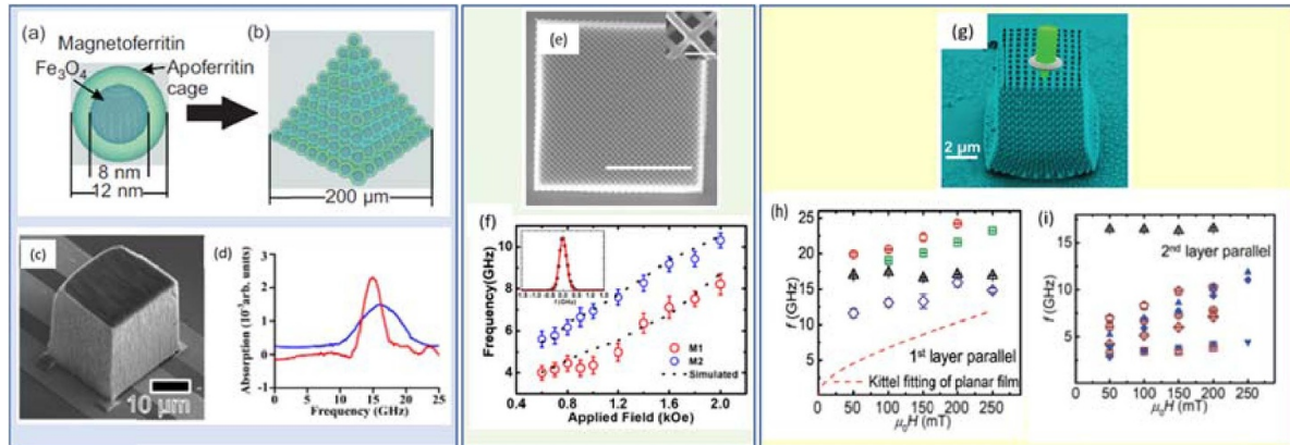
Figure 27. (a) Sketch of a single apoferritin cage with magnetite ( \text{Fe}_3\text{O}_4 ) nanoparticle enclosed in its cavity. (b) Under appropriate conditions the nanoparticle arrange into a regular fcc lattice via self organization. (c) SEM image of a cubic \text{Fe}_3\text{O}_4 -ferritin crystal fabricated by FIB fixed to the two outer ground lines of a coplanar waveguide. (d) Microwave absorption spectra taken in an external magnetic field of 0.5 T applied in a direction perpendicular to the substrate (red line: 290 K, blue line: 5 K). Reproduced from [175]. © IOP Publishing Ltd All rights reserved. (e) SEM image of the full array of artificial spin-ice and (f) the dependence of modes frequencies on the applied magnetic field. Reproduced from [92]. CC BY 4.0. (g) SEM image of the 3D Ni nanowire nanonetwork (woodpile structure) and frequency dependence of modes when the applied field is parallel to the (h) first and (i) to the second layer of the woodpile structure. Reproduced from [23]. CC BY 4.0.
