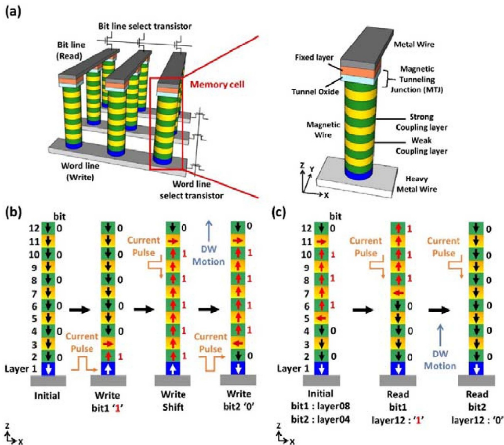
Figure 33. (a) Illustration of the vertical DW motion memory with artificial ferromagnets. Left panel: Memory array with vertically arranged word line and bit line. The columns within the array are the multi-bit memory cells constructed with artificial ferromagnets. Right panel: Detailed structure of a column. (b) Data writing scheme: A current is applied to the bottom electrode to invert the magnetization direction of layer 1 by spin-orbit torque. A DW is then generated in layer 3. The current is then passed through the column to shift this DW up to any DW layer. The next information is then written by inverting the magnetization direction of layer 1 by applying a current to the bottom electrode. By repeating this operation, any bit sequence can be stored in the column. (c) Readout can be done in batches by reading out the information at the top MTJ while shifting all DWs upwards with a current. Reproduced from [194]. CC BY 4.0.
