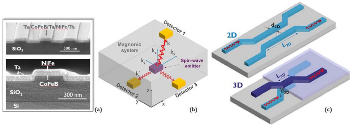
Figure 28. (a) Scanning Electron Microscope images of a three-dimensional nanoscale CoFeB/Ta/NiFe meander structure. Reproduced from [182]. CC BY 4.0. (b) Schematic of a 3D magnonic system where the 3D character of the spin-wave wavevector selects the receiving detector. (c) Comparison of 2D and 3D magnonic directional couplers based on waveguides made from thin films. The most relevant parameter for miniaturization and energy consumption is the coupling length L . Due to the much smaller waveguide distance d_{3D} \ll d_{2D} and the larger surface overlap in the 3D case, the coupling length L_{3D} is generally much smaller than L_{2D} . In 3D, the potential use of the exchange interaction to couple the energy between the two waveguides provides also a much more favorable scaling towards higher frequencies/smaller wavelengths.
