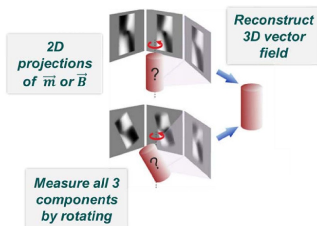
Figure 10. The principles of 3D magnetic nanoimaging. Two-dimensional transmission projections of the magnetic induction \vec{B} (electron imaging) or the magnetization \vec{m} (x-ray magnetic circular dichroism imaging) are acquired at several different angles by rotating the sample for many different orientations of the sample with respect to the probe beam. While only two are shown here, sufficient sample orientations should be acquired to ensure that all components of the vector field are sufficiently sampled. The final three-dimensional magnetic induction or magnetization vector field is then reconstructed using a dedicated reconstruction algorithm. Schematic reproduced from [63]. © IOP Publishing Ltd CC BY 3.0.
