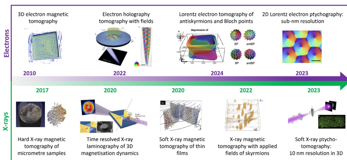
Figure 11. Developments in 3D magnetic nanoimaging, with milestones in both electron (upper panel) and x-ray (lower panel) 3D imaging shown over the years. Reproduced from [57]. CC BY 4.0. Reproduced from [60], with permission from Springer Nature. Reproduced from [61]. CC BY 4.0. Reproduced from [62], with permission from Springer Nature. Reprinted (figure) with permission from [64], Copyright (2010) by the American Physical Society. Reproduced from [65]. CC BY 4.0. Reproduced from [66], with permission from Springer Nature. Reproduced from [67], with permission from Springer Nature. Reproduced from [68], with permission from Springer Nature.
