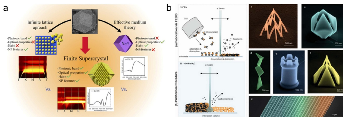
Figure 17. (a) Approaches to calculate the properties of photonic crystals, i.e. infinite lattice for band structure calculations, effective medium theory for optical properties like reflectance, and proposed FDTD simulation for finite supercrystals. (b) Fabrication, purification, and 3D possibilities. Top-left side: a gas injection system (GIS) injects preheated precursor molecules in gaseous states ( \text{Me}_2(\text{acac})\text{Au}(\text{III}) in this study) in close proximity to the substrate, where they adsorb, diffuse and, if not dissociated, eventually desorb again. Upon interaction with a focused electron beam, local dissociation leads to immobilization of the respective metal, which forms the intended deposit. As a result of incomplete ligand cleavage not only Au atoms (orange spheres) but also carbonaceous fragments (grey spheres) are co-deposited, which is why FEBID structures naturally contain high amounts of carbon. The whole fabrication procedure is typically performed at 21 \pm 1^\circ\text{C} and 10–5 Pa. Right panel: 3D nano-printing design possibilities, ranging from meshed objects over sheet-like, semi-closed toward closed and mixed architectures. Also, scalability is provided, to generate micrometre-sized assemblies for individual applications (see tetrapod array). To remove the carbon, the scheme on the bottom-left panel illustrates a suitable purification process, which takes place in a low-pressure \text{H}_2\text{O} atmosphere ranging between 50–100 Pa at 21 \pm 1^\circ\text{C} . Using again the focused electron beam leads to the local removal of carbon, leaving nominally pure, polycrystalline gold nanostructures with a volume loss of up to two thirds. Depending on the height of the nanostructure, the beam conditions must be adapted such that the interaction volume can cover the whole structure volume. Panel (a) is reproduced from [106] with permission from the Royal Society of Chemistry. Panel (b) is [109] John Wiley & Sons. [Copyright © 2023 WILEY-VCH Verlag GmbH & Co. KGaA, Weinheim].
