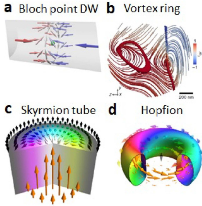
Figure 18. Schematic spin textures of (a) a Bloch point type domain wall. Reproduced from [6]. CC BY 4.0. (b) Vortex ring. Reproduced from [7], with permission from Springer Nature. (c) A skyrmion tube, and (d) a Hopfion with Hopf index = 1. Reproduced from [8]. CC BY 4.0.
