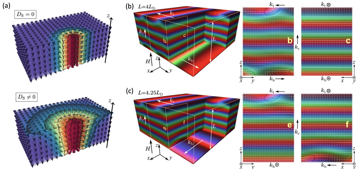
Figure 24. (a) Magnetic edge surface states induced by the correct boundary conditions in chiral thin semi-infinite films with bulk DMI. Reprinted (figure) with permission from [159], Copyright (2018) by the American Physical Society. By including the symmetric elements of the DMI tensor in the boundary conditions, additional terms appear, increasing the skyrmion radius near the surface. (b), (c) Bulk DMI in thick films with free boundary conditions and distinctive surface magnetic states. Reproduced from [157]. © IOP Publishing Ltd CC BY 3.0. In the bulk there is a helical state along the field, while at the top and bottom surfaces, the direction of the helix changes depending on the film thickness.
