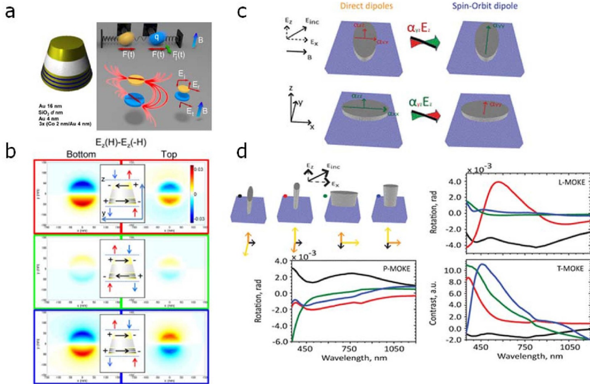
Figure 16. (a) Left panel: schematic drawing of the nanoresonators composed of a purely plasmonic Au disk and a magnetoplasmonic Au/Co superlattice disk separated by a dielectric spacer. Top-right panel: spring model representing a two coupled masses system excited by a harmonic force, F(t) , along x axis. One of the masses (blue) is charged ( q ) and a static magnetic field ( B ) is applied along the z direction, inducing a Lorentz force, F_1(t) , along the y direction. The y -movement is transferred to the other mass through the coupling. Bottom-right panel: two interacting electric dipoles, representing two metallic disks, excited by an incident beam polarized along the x axis. One of the disks (blue) has magneto-optical activity and a static magnetic field ( B ) applied along the z direction induces a rotation of its electric dipole, which is transferred to the other dipole through the interaction. The rotation modifies the polarization direction of the reflected ( E_r ) and transmitted ( E_t ) light. (b) Difference of the E_z components for magnetic saturation along opposite directions in the same planes and for the same structure. This difference accounts for the effect of the applied magnetic field: the appearance of a dipole along the y direction for both the magnetoplasmonic (intrinsic dipole) and the plasmonic (induced dipole) disks. In both cases, the components for three different wavelengths labelled with different colours (red, green, and blue frames). At specific frequencies (e.g. see green frame) the magneto-optical response is suppressed due to the destructive interference between the two dipoles. (c) Schematic overview of the interplay of the directly excited (left, resonant \alpha_{xx} and off-resonant \alpha_{zz} ) and spin-orbit coupled (right, resonant \alpha_{yy} ) nanoantenna modes that all together deliver exceptional light polarization rotation control. Light incidence ( p -polarized) and applied magnetic field are marked. (d) Schematic set of 3D nanoantennas (top, left) with highlighted dipolar on (yellow, orange)/off (grey) resonance modes. p -polarized light is always used. Calculated Kerr signals for the nanoantennas in panel in L-MOKE (top, right), P-MOKE (bottom, right), and T-MOKE (bottom, left). Panels (a) and (b) are reprinted with permission from [97] © Optica Publishing Group. Panels (c) and (d) are reprinted with permission from [100]. Copyright (2014) American Chemical Society.
