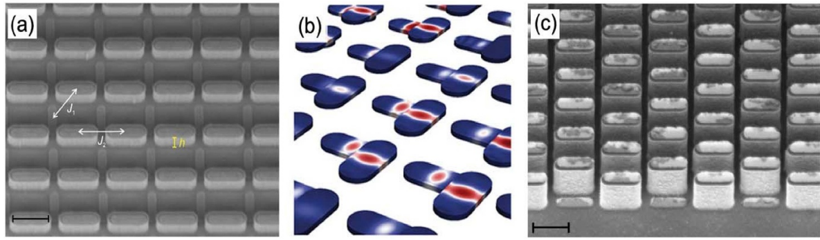
Figure 14. (a) Quasi-3D artificial spin ice realized by placing Ising-type nanomagnets on top of pre-etched silicon substrates. The etching depth defines the achieved height offset that allows the tuning of the balance between competing interactions J_1 and J_2 and the realization of macroscopic spin ice degeneracy. It also serves as a basis for novel 3D magnonic crystals (b). (c) Artificial planar triangular antiferromagnet, a concept that could not be realized within the 2D constraints. Scale bar in (a), (c) is 400 nm. (a) Reproduced from [89]. CC BY 4.0. (b) Reproduced from [88]. CC BY 4.0.
