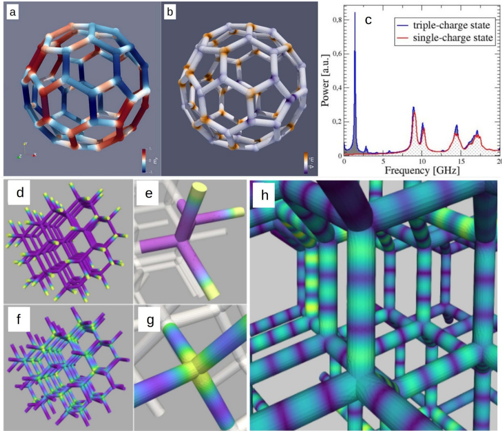
Figure 25. Simulated high-frequency magnetization dynamics in interconnected nanowire array geometries. The finite-element method allows for an accurate representation of the complex shape. Panels (a) and (b) show the static magnetization structure in a buckyball-type nanoarchitecture and its configuration-dependent oscillation spectrum, simulated in the time domain with the ringdown method (c). Reprinted from [165], with the permission of AIP Publishing. Panels (d)–(h) show various oscillation modes in a diamond-type artificial magnetic crystal developing at different frequencies. See [9] for details. Panels (d)–(h) are reproduced with permission from [9].
