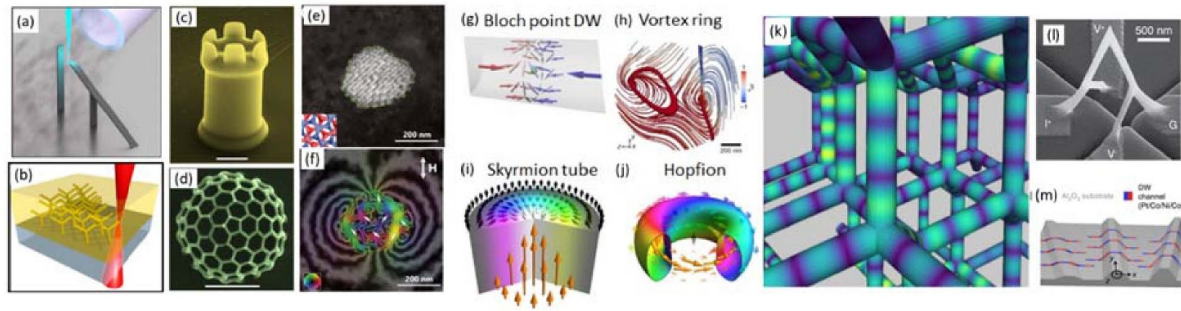
Figure 1. (a) Focused electron beam induced deposition (FEED). Reproduced from [1]. CC BY 4.0. (b) Two-photon lithography method. Reproduced from [2]. CC BY 4.0. By the controlled beam movement, bulky (c) and complex buckyball like (d) structures can be realized using FEED. Reproduced with permission from [3]. Reproduced from [4]. CC BY 4.0. Phase contrast imaging with off-axis and in-line electron holography using aberration-corrected transmission electron microscopy. (e) Structure and (f) magnetic induction of 3D gyroid network visualized with off-axis holography. Reprinted with permission from [5]. Copyright (2020) American Chemical Society. Schematic spin textures of (g) a Bloch point type domain wall. Reproduced from [6]. CC BY 4.0. (h) vortex ring. Reproduced from [7], with permission from Springer Nature. (i) a skyrmion tube, and (j) a Hopfion with Hopf\ index = 1 . Reproduced from [8]. CC BY 4.0. (k) Various oscillation modes in a diamond-type artificial magnetic crystal developing at different frequencies. Reproduced with permission from [9]. Exemplary 3D spintronics devices showing (l) ferromagnetic interconnector directly printed by FEED. Reproduced from [10]. CC BY 4.0. (m) State-of-the-art racetrack memories formed by synthetic antiferromagnets, positioned on 3D pre-patterned substrates to achieve vertical domain wall motion. Reproduced from [11]. CC BY 4.0.
