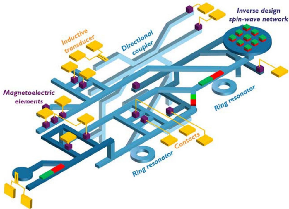
Figure 29. Schematic view of a potential 3D magnonic network consisting of 2D layers connected by 3D directional couplers. Different elements like inductive transducers and magneto-electric elements (for spin wave excitation and phase shift), permanent magnets (for reconfiguration), ring resonators (filtering) and an area for inverse design are shown.
